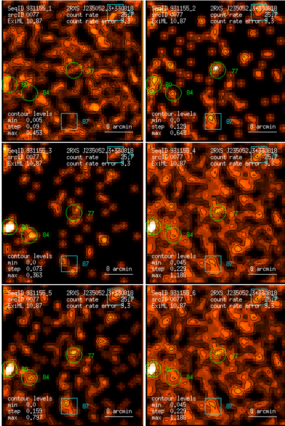
Figure 77: RASS 931155: detection 0077: band rate images, Gaussian filter: (1) PSPC channels 11 – 41, (2) 52 – 90, (3) 91 – 201, (4) 11 – 235, (5) 52 – 201, (6) 11 – 201. Broad band rates in counts/ks. Band rate contour levels in counts/ks/arcmin 2 .
