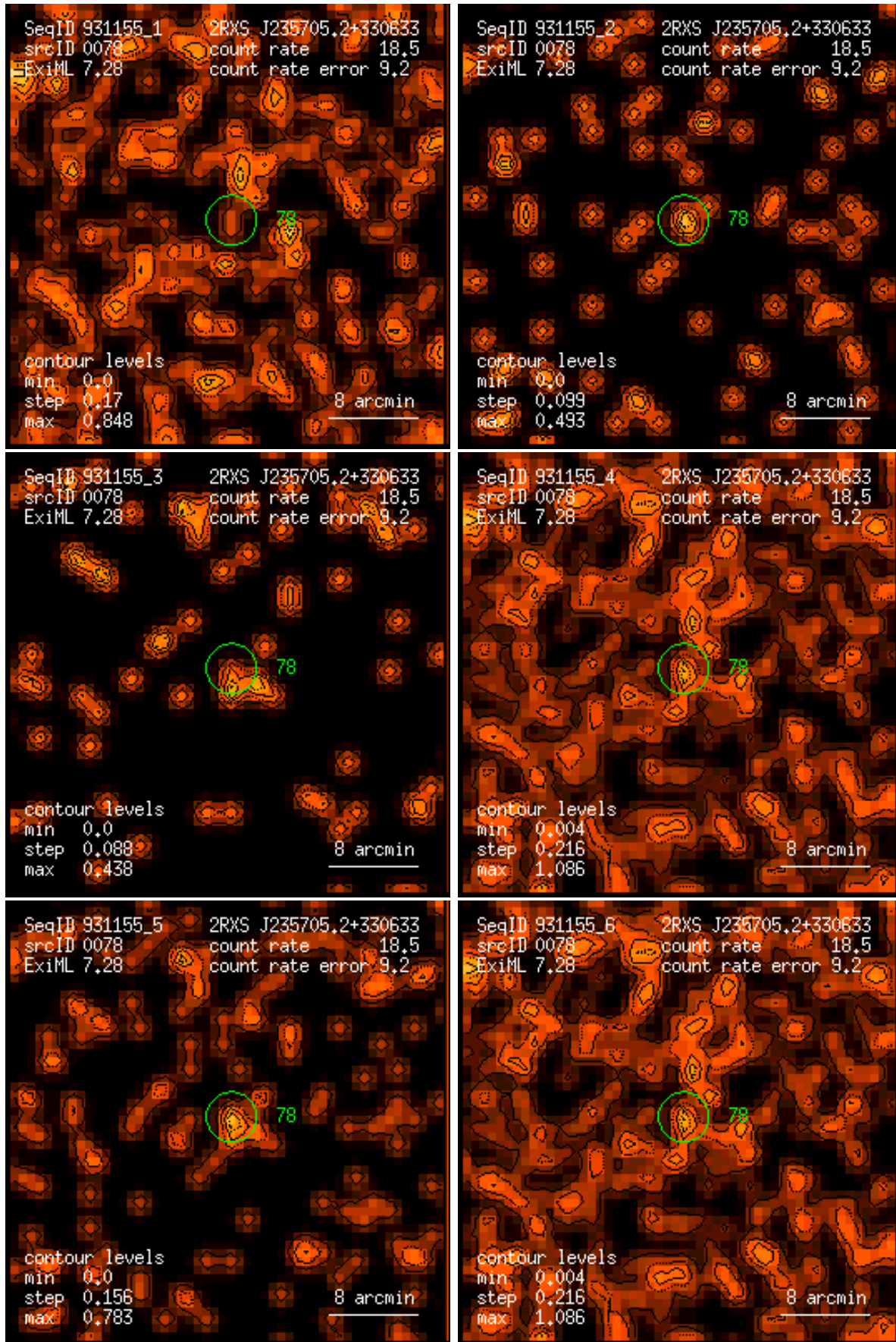
Figure 78: RASS 931155: detection 0078: band rate images, Gaussian filter: (1) PSPC channels 11 – 41, (2) 52 – 90, (3) 91 – 201, (4) 11 – 235, (5) 52 – 201, (6) 11 – 201. Broad band rates in counts/ks. Band rate contour levels in counts/ks/arcmin 2 .
