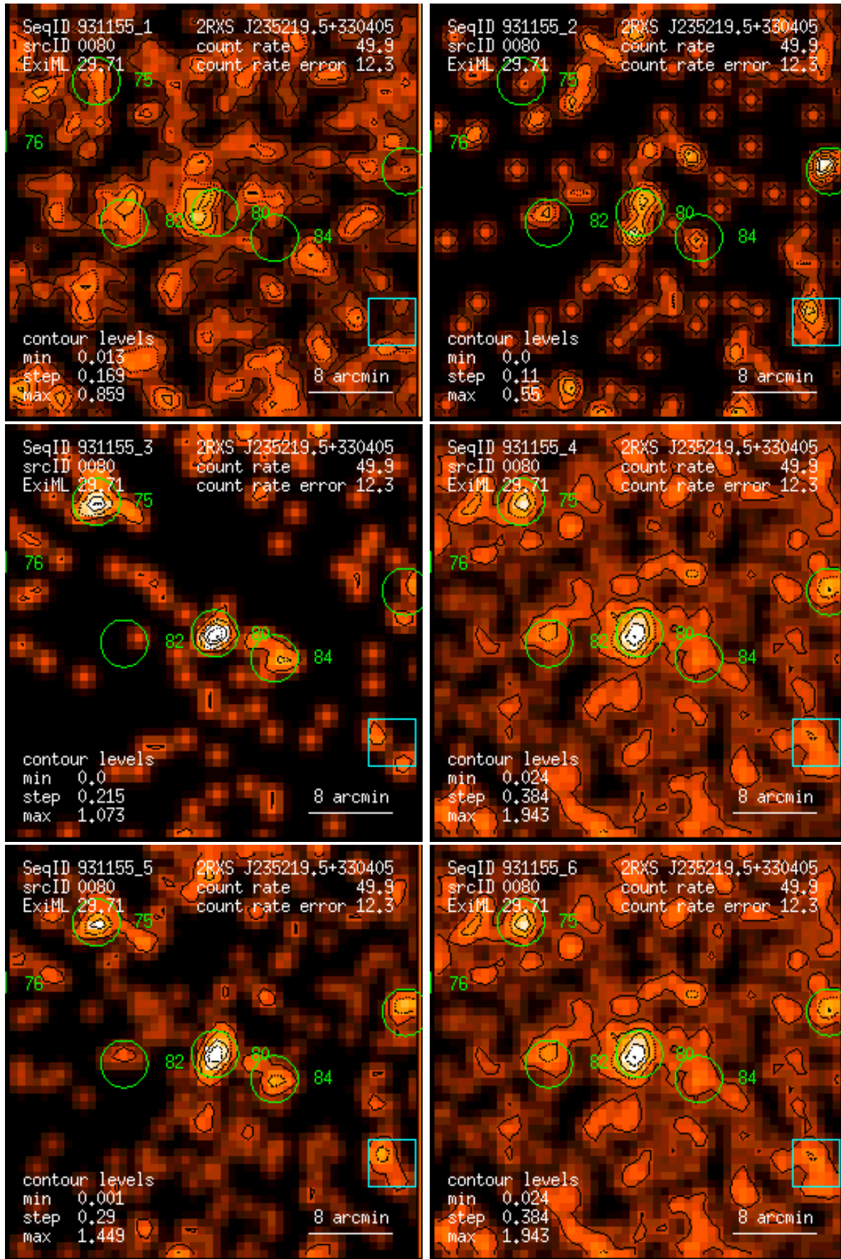
Figure 80: RASS 931155: detection 0080: band rate images, Gaussian filter: (1) PSPC channels 11 – 41, (2) 52 – 90, (3) 91 – 201, (4) 11 – 235, (5) 52 – 201, (6) 11 – 201. Broad band rates in counts/ks. Band rate contour levels in counts/ks/arcmin 2 .
