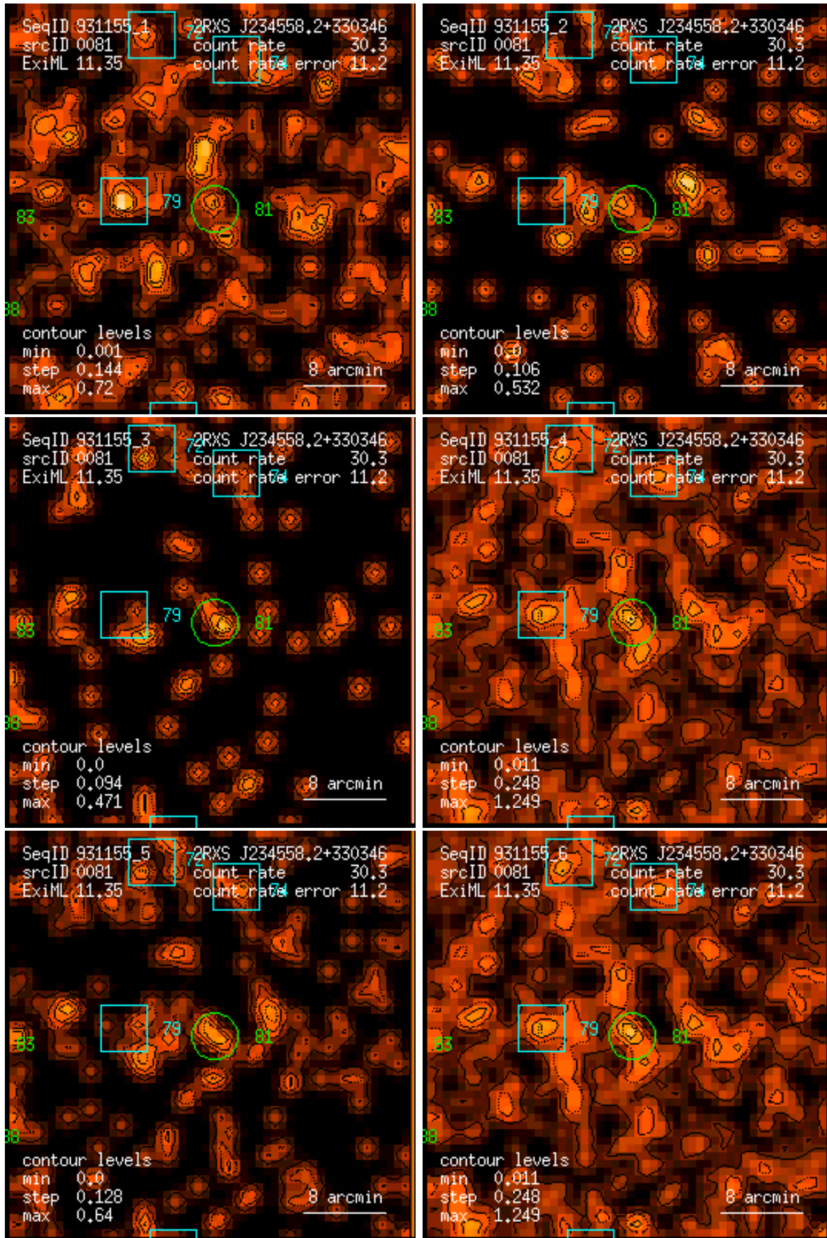
Figure 81: RASS 931155: detection 0081: band rate images, Gaussian filter: (1) PSPC channels 11 – 41, (2) 52 – 90, (3) 91 – 201, (4) 11 – 235, (5) 52 – 201, (6) 11 – 201. Broad band rates in counts/ks. Band rate contour levels in counts/ks/arcmin 2 .
