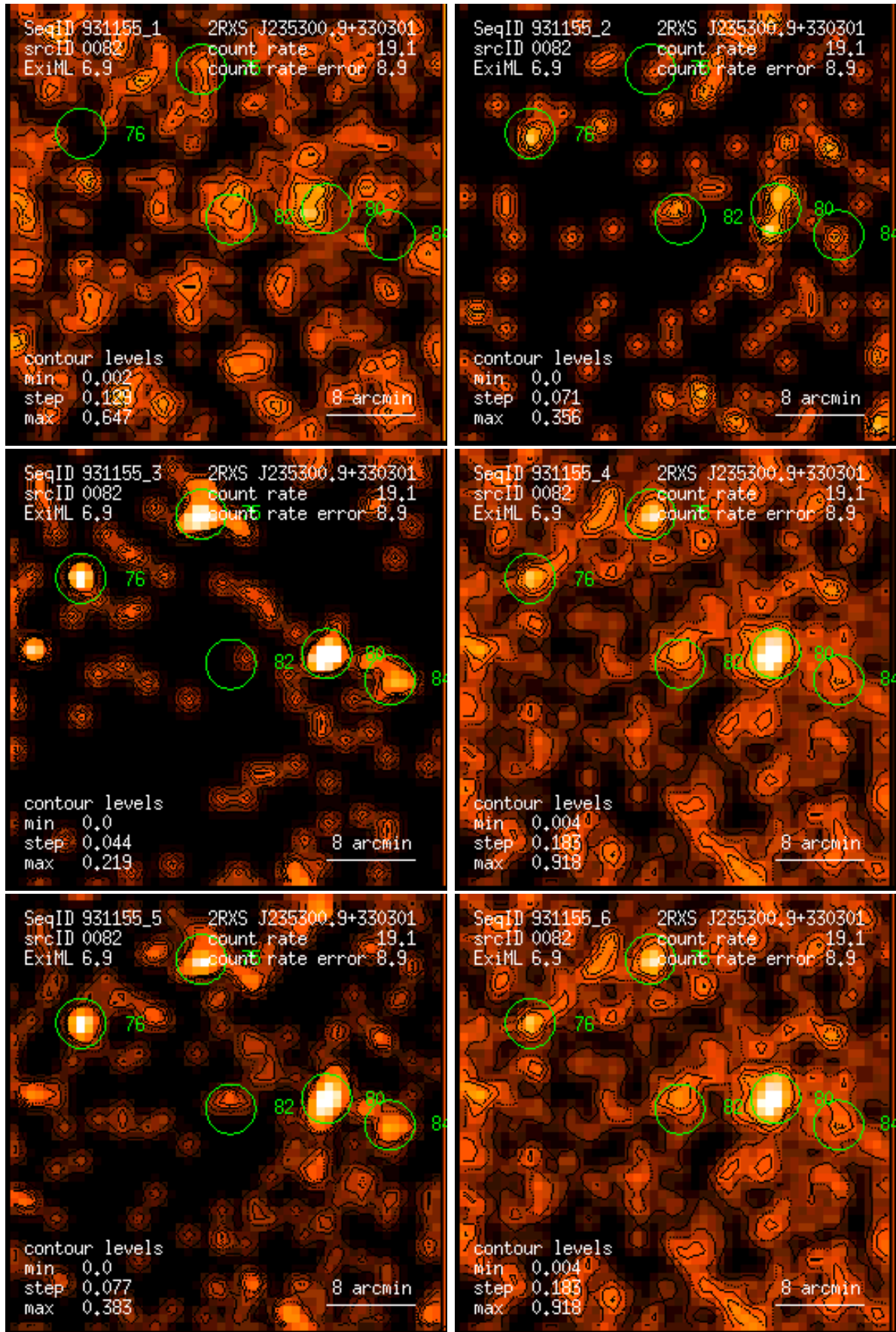
Figure 82: RASS 931155: detection 0082: band rate images, Gaussian filter: (1) PSPC channels 11 – 41, (2) 52 – 90, (3) 91 – 201, (4) 11 – 235, (5) 52 – 201, (6) 11 – 201. Broad band rates in counts/ks. Band rate contour levels in counts/ks/arcmin 2 .
