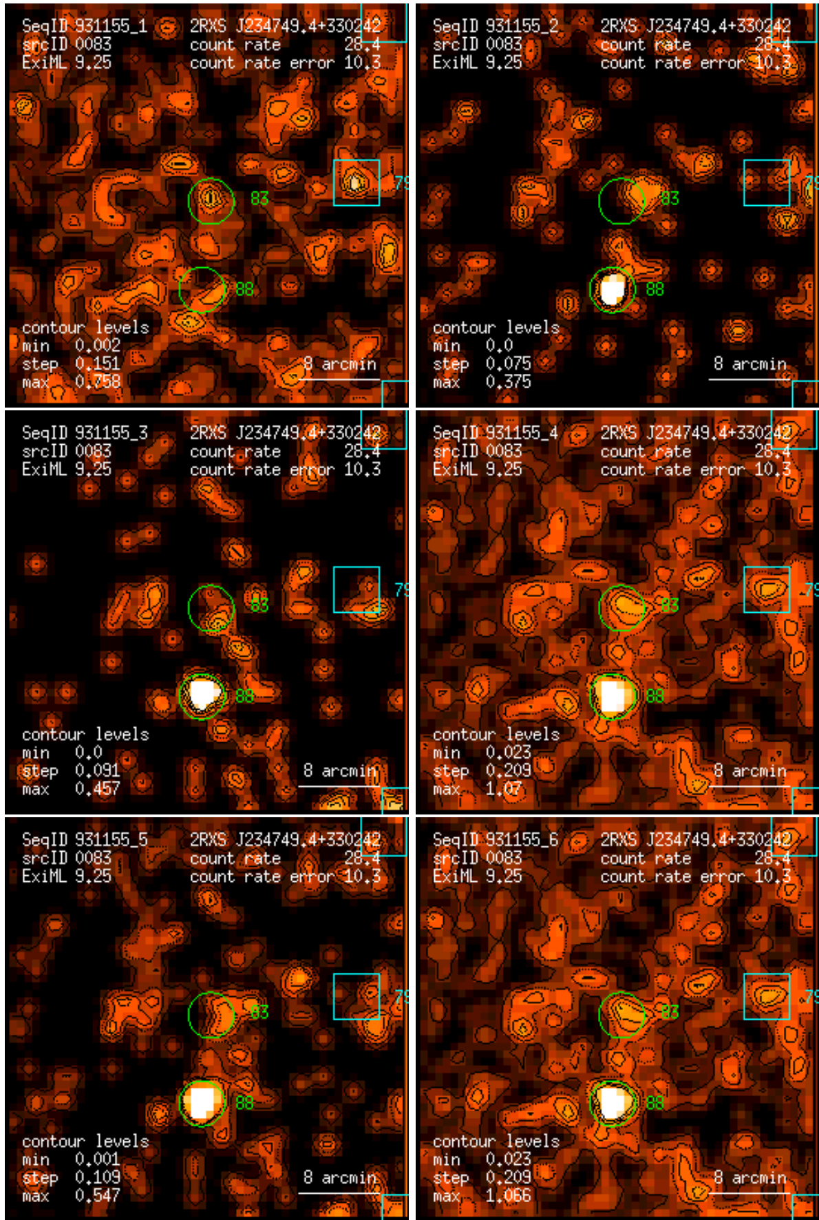
Figure 83: RASS 931155: detection 0083: band rate images, Gaussian filter: (1) PSPC channels 11 – 41, (2) 52 – 90, (3) 91 – 201, (4) 11 – 235, (5) 52 – 201, (6) 11 – 201. Broad band rates in counts/ks. Band rate contour levels in counts/ks/arcmin 2 .
