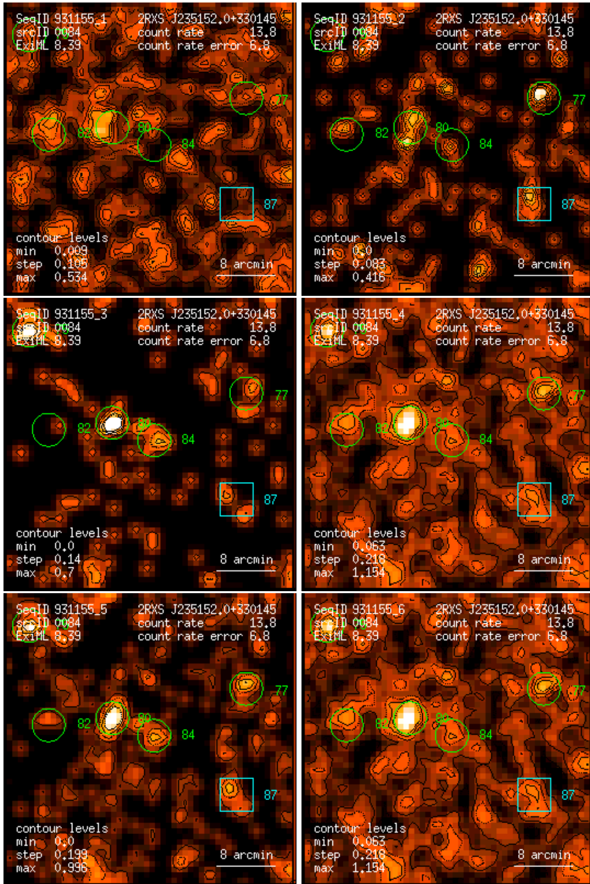
Figure 84: RASS 931155: detection 0084: band rate images, Gaussian filter: (1) PSPC channels 11 – 41, (2) 52 – 90, (3) 91 – 201, (4) 11 – 235, (5) 52 – 201, (6) 11 – 201. Broad band rates in counts/ks. Band rate contour levels in counts/ks/arcmin 2 .
