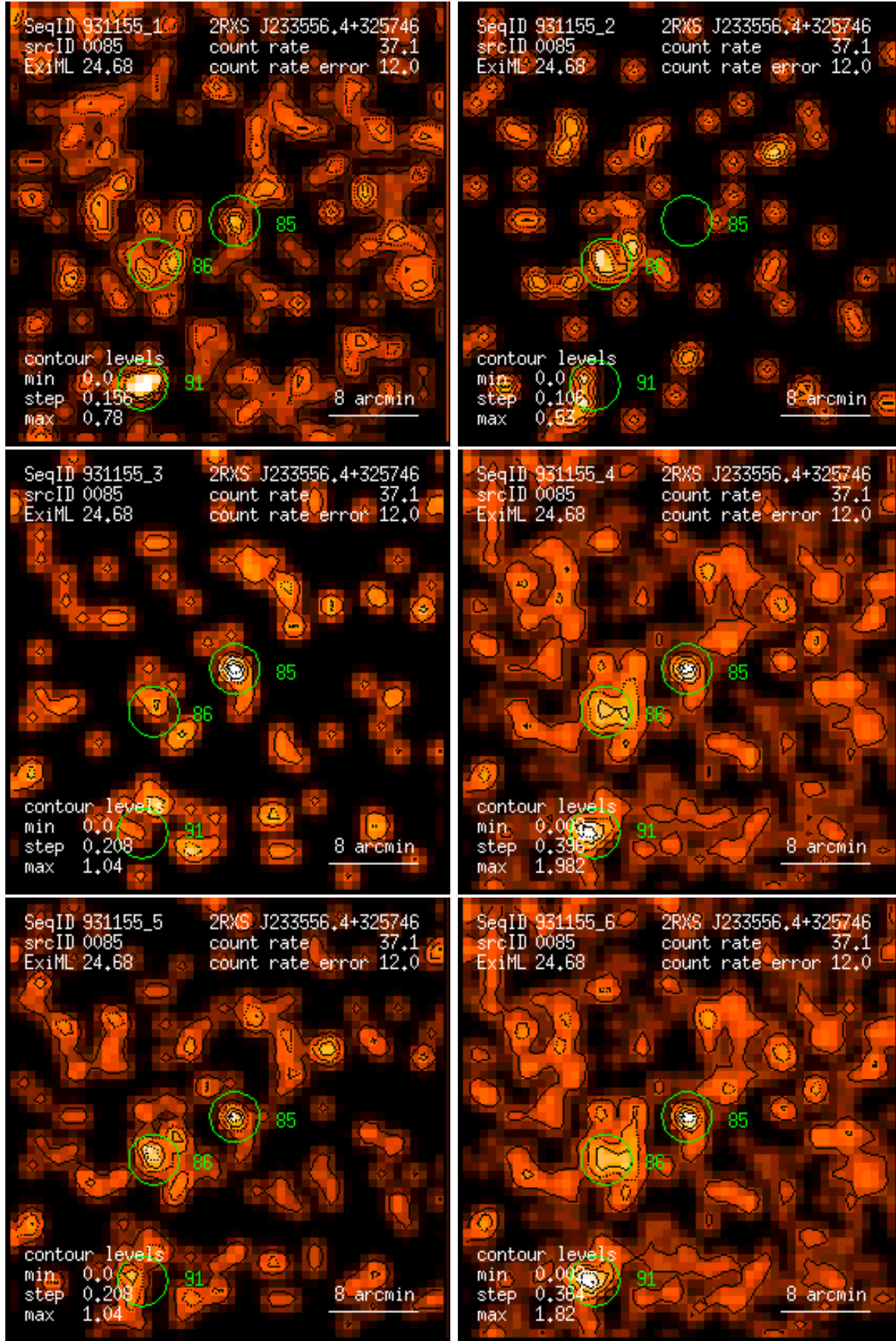
Figure 85: RASS 931155: detection 0085: band rate images, Gaussian filter: (1) PSPC channels 11 – 41, (2) 52 – 90, (3) 91 – 201, (4) 11 – 235, (5) 52 – 201, (6) 11 – 201. Broad band rates in counts/ks. Band rate contour levels in counts/ks/arcmin 2 .
