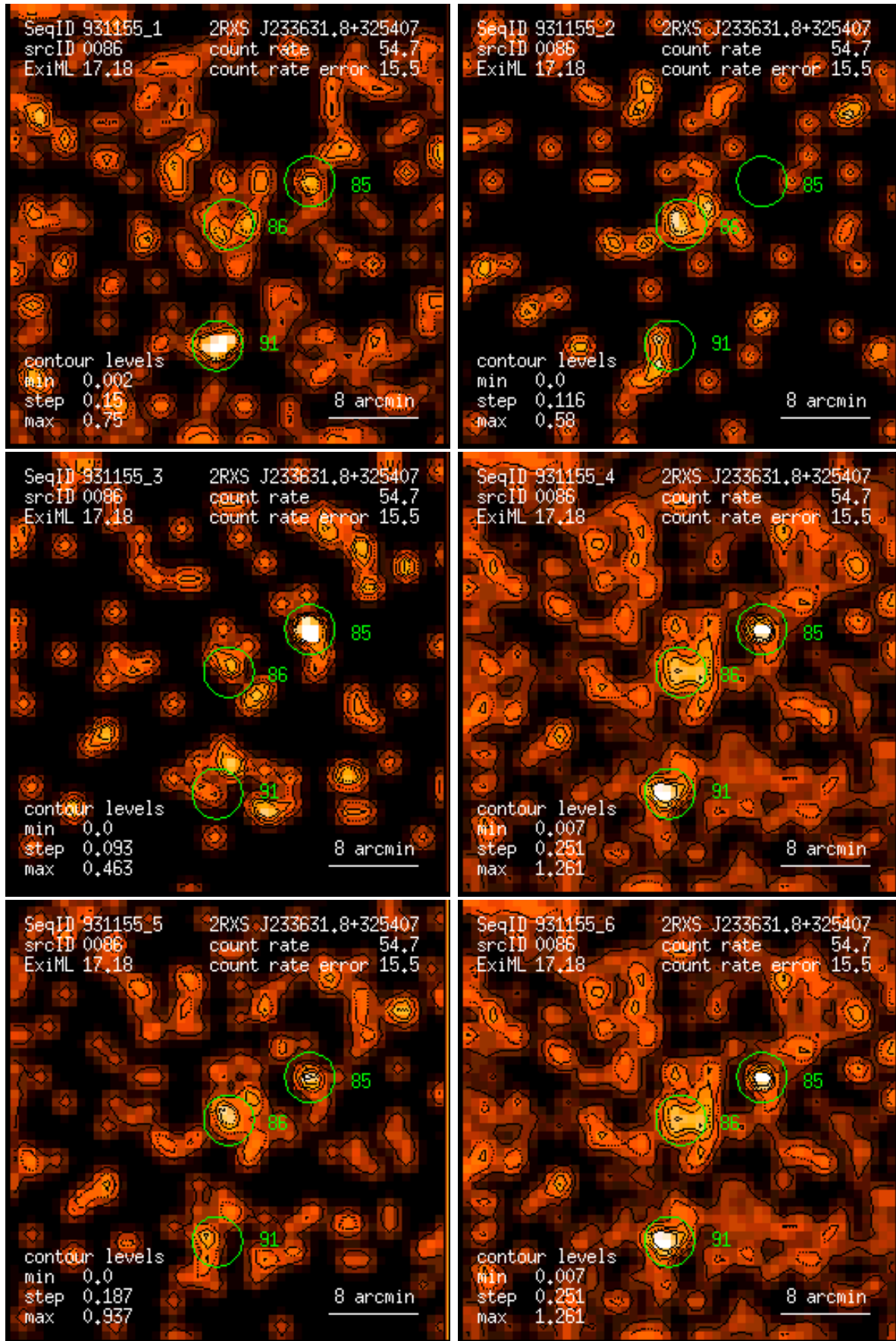
Figure 86: RASS 931155: detection 0086: band rate images, Gaussian filter: (1) PSPC channels 11 – 41, (2) 52 – 90, (3) 91 – 201, (4) 11 – 235, (5) 52 – 201, (6) 11 – 201. Broad band rates in counts/ks. Band rate contour levels in counts/ks/arcmin 2 .
