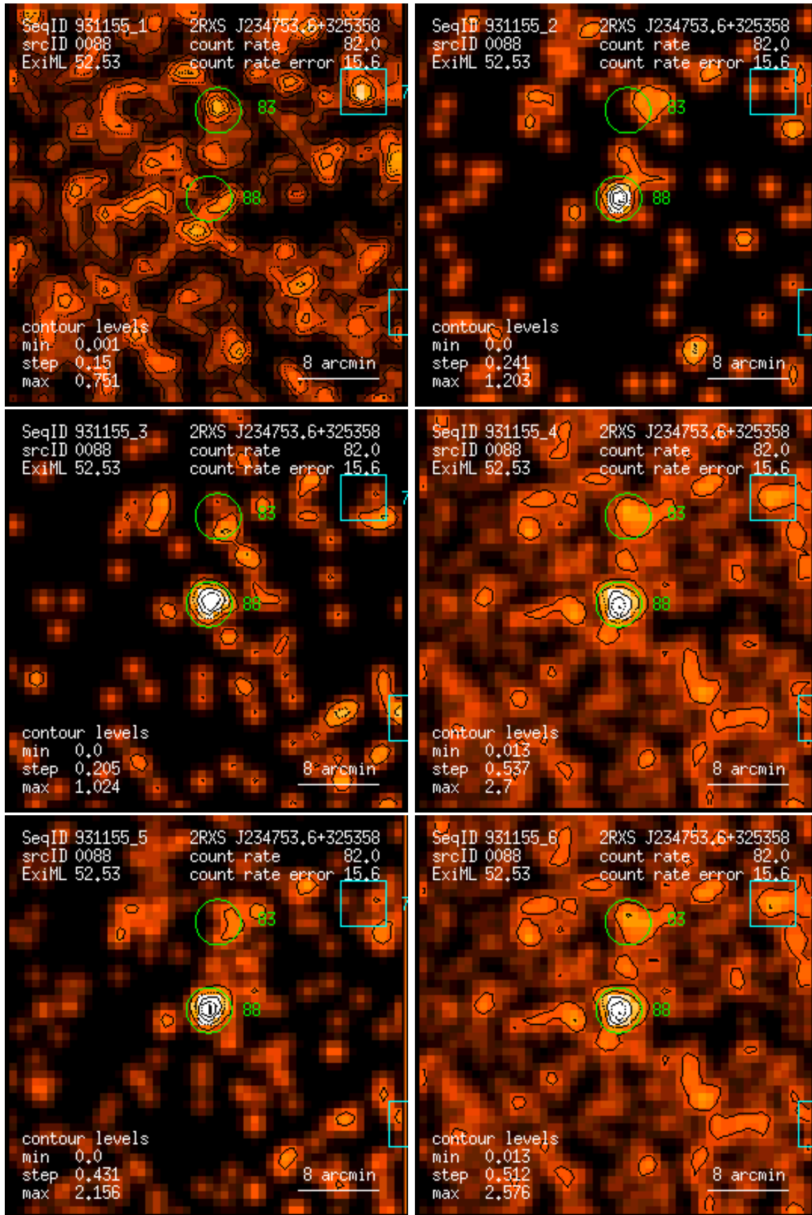
Figure 88: RASS 931155: detection 0088: band rate images, Gaussian filter: (1) PSPC channels 11 – 41, (2) 52 – 90, (3) 91 – 201, (4) 11 – 235, (5) 52 – 201, (6) 11 – 201. Broad band rates in counts/ks. Band rate contour levels in counts/ks/arcmin 2 .
