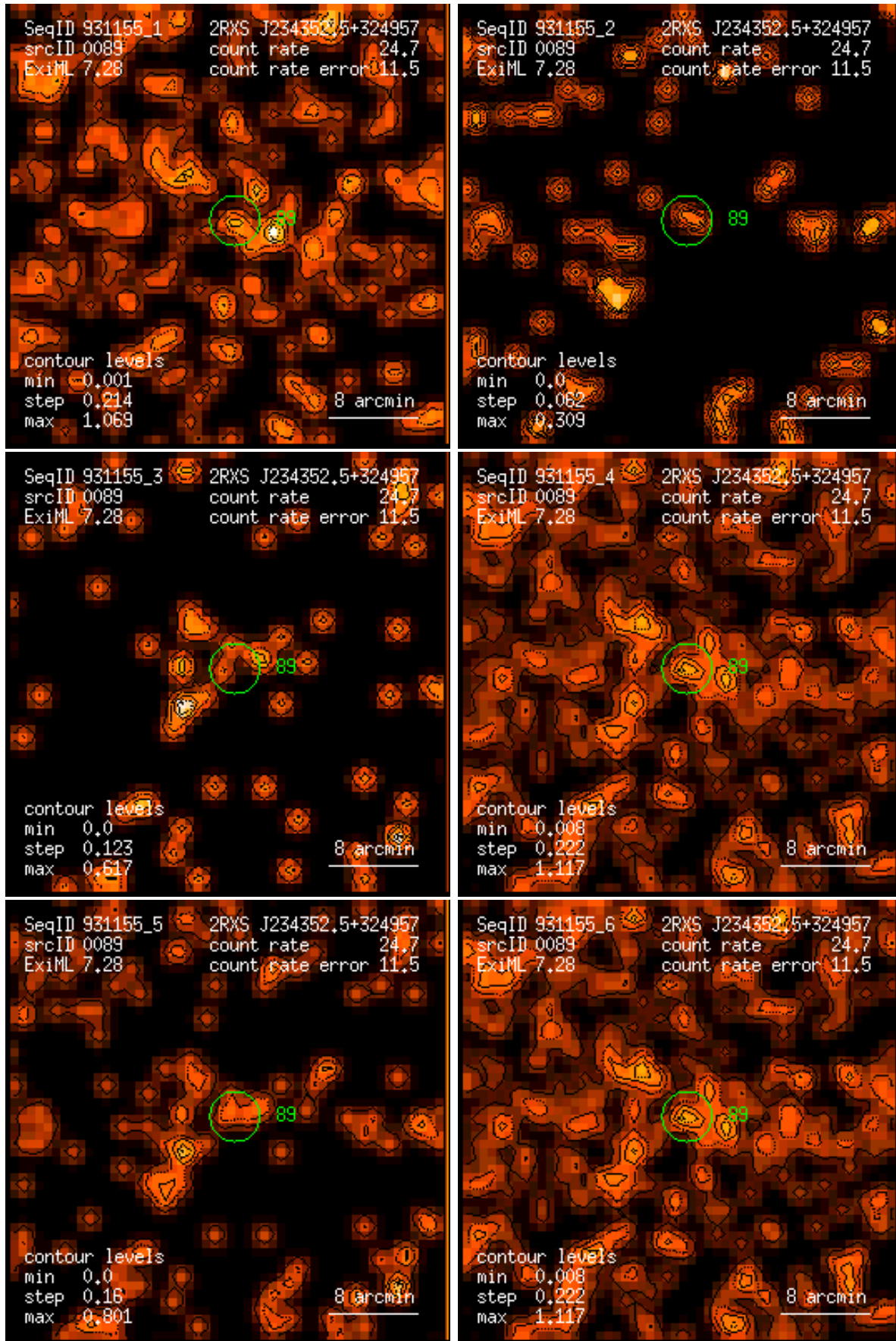
Figure 89: RASS 931155: detection 0089: band rate images, Gaussian filter: (1) PSPC channels 11 – 41, (2) 52 – 90, (3) 91 – 201, (4) 11 – 235, (5) 52 – 201, (6) 11 – 201. Broad band rates in counts/ks. Band rate contour levels in counts/ks/arcmin 2 .
