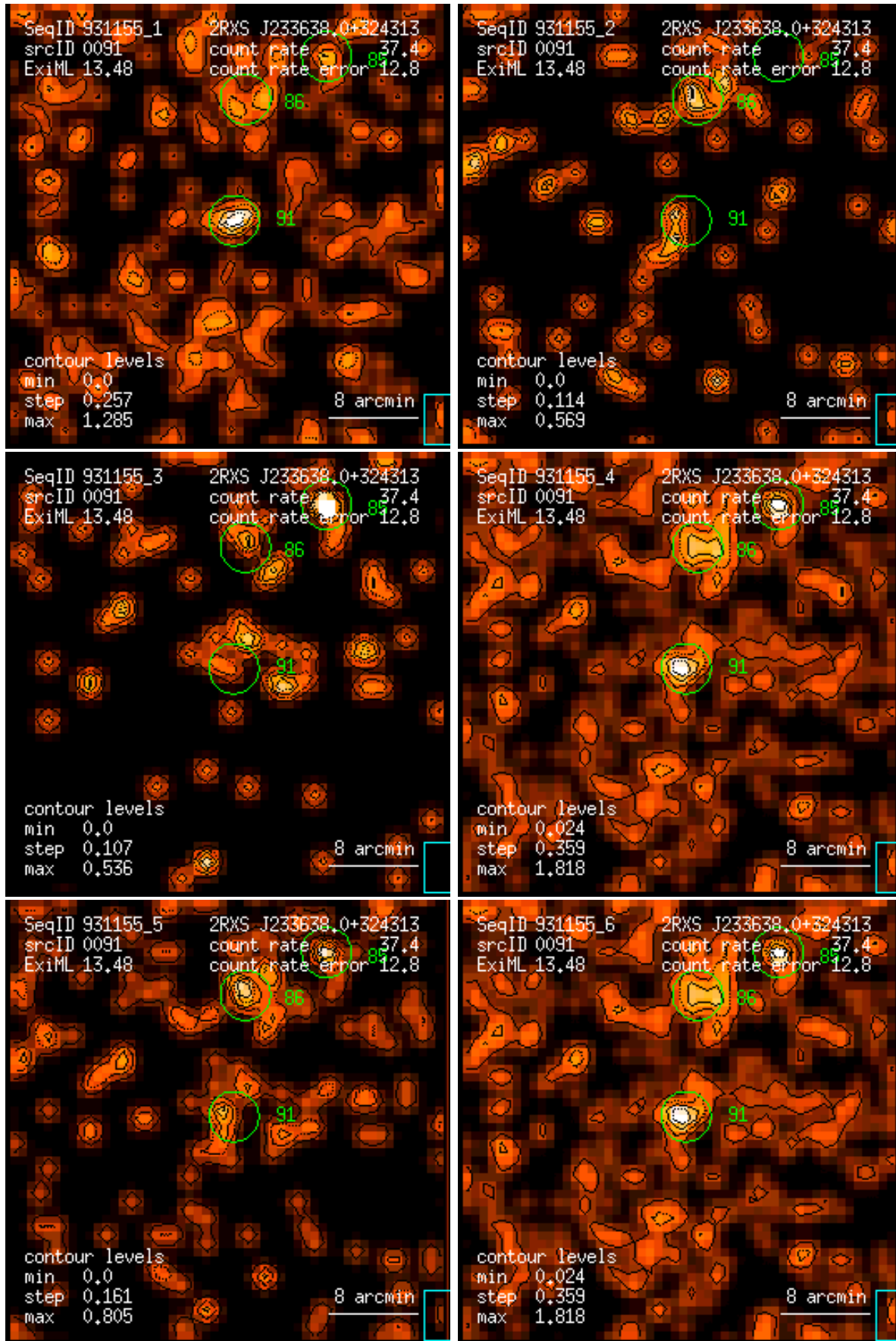
Figure 91: RASS 931155: detection 0091: band rate images, Gaussian filter: (1) PSPC channels 11 – 41, (2) 52 – 90, (3) 91 – 201, (4) 11 – 235, (5) 52 – 201, (6) 11 – 201. Broad band rates in counts/ks. Band rate contour levels in counts/ks/arcmin 2 .
