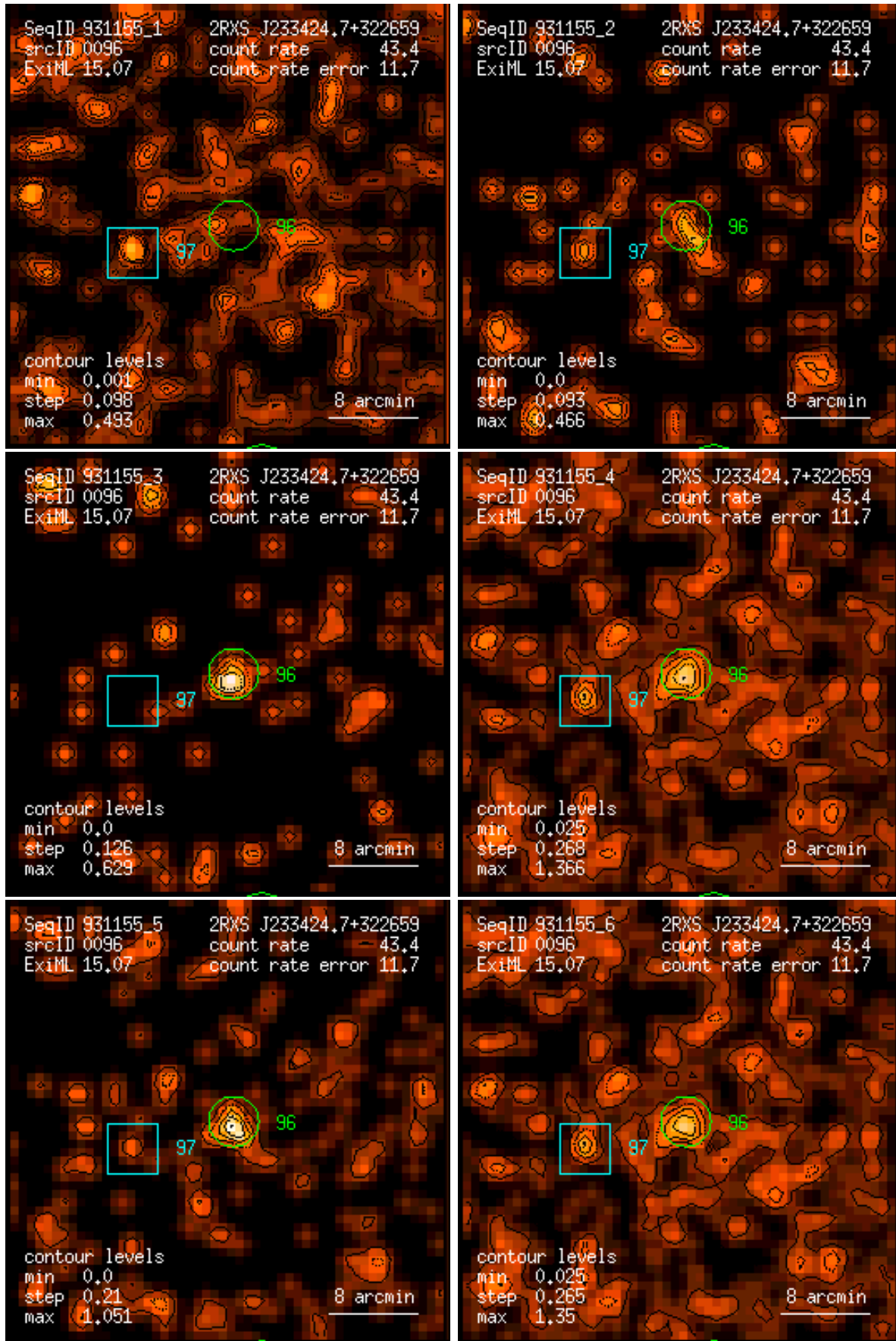
Figure 96: RASS 931155: detection 0096: band rate images, Gaussian filter: (1) PSPC channels 11 – 41, (2) 52 – 90, (3) 91 – 201, (4) 11 – 235, (5) 52 – 201, (6) 11 – 201. Broad band rates in counts/ks. Band rate contour levels in counts/ks/arcmin 2 .
