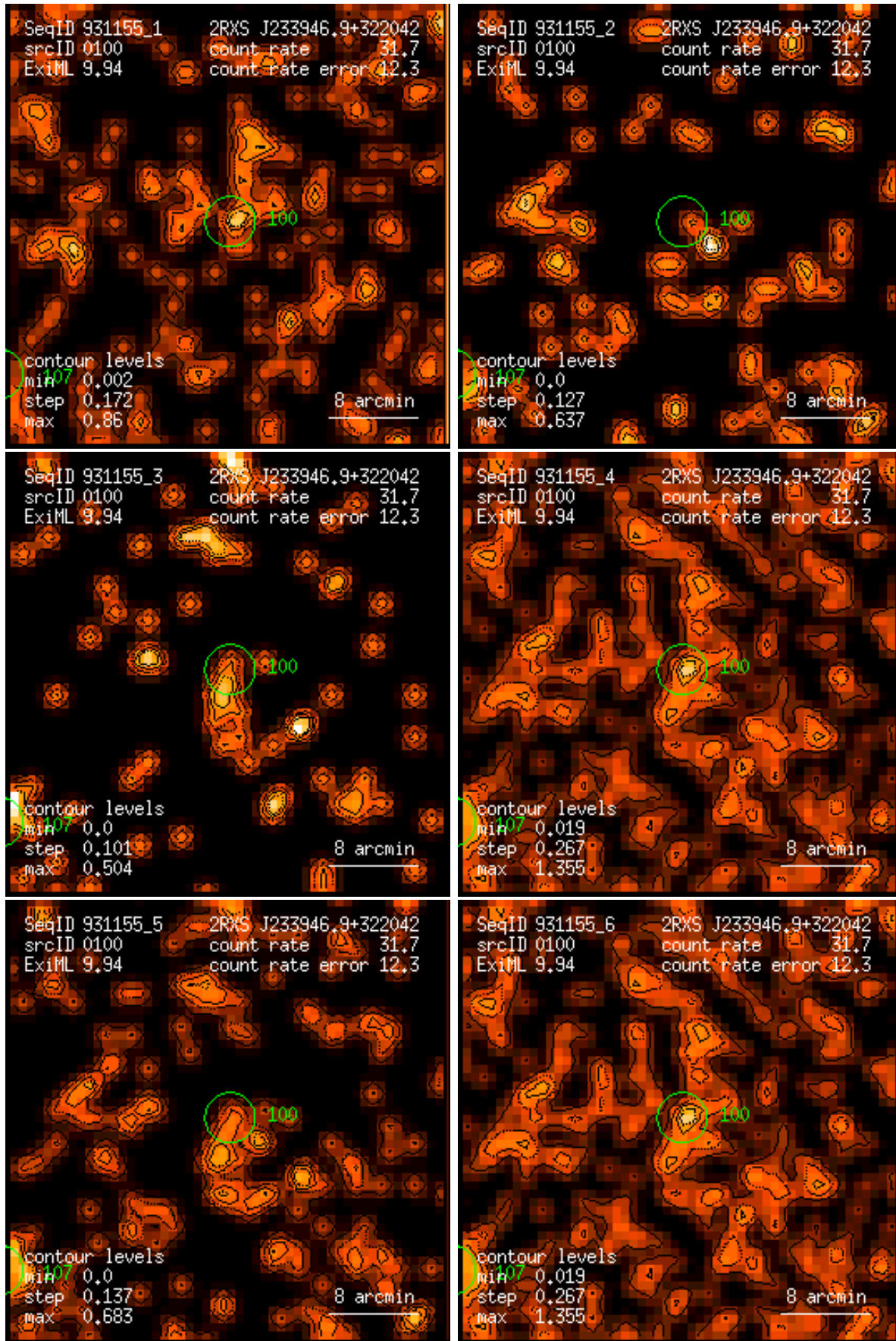
Figure 100: RASS 931155: detection 0100: band rate images, Gaussian filter: (1) PSPC channels 11 – 41, (2) 52 – 90, (3) 91 – 201, (4) 11 – 235, (5) 52 – 201, (6) 11 – 201. Broad band rates in counts/ks. Band rate contour levels in counts/ks/arcmin 2 .
