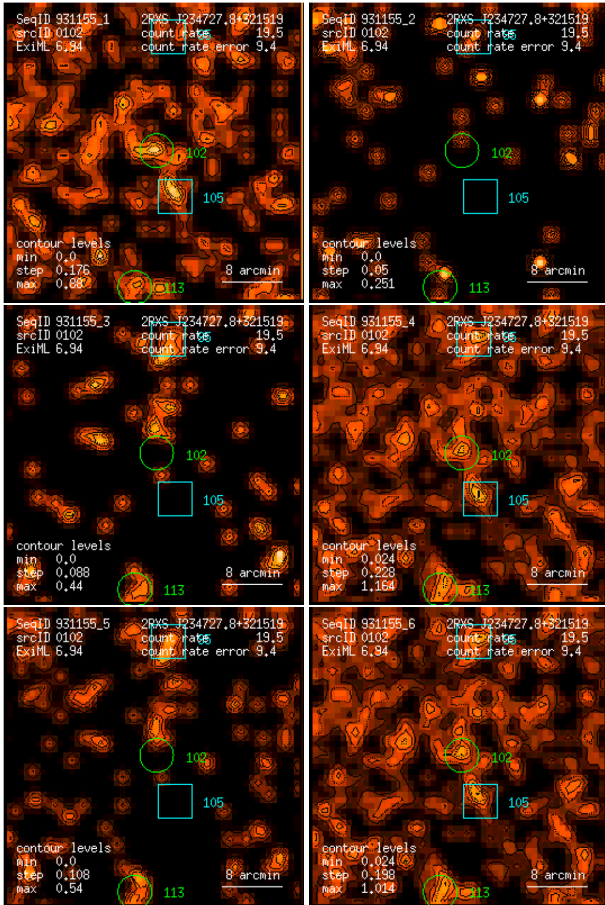
Figure 102: RASS 931155: detection 0102: band rate images, Gaussian filter: (1) PSPC channels 11 – 41, (2) 52 – 90, (3) 91 – 201, (4) 11 – 235, (5) 52 – 201, (6) 11 – 201. Broad band rates in counts/ks. Band rate contour levels in counts/ks/arcmin 2 .
