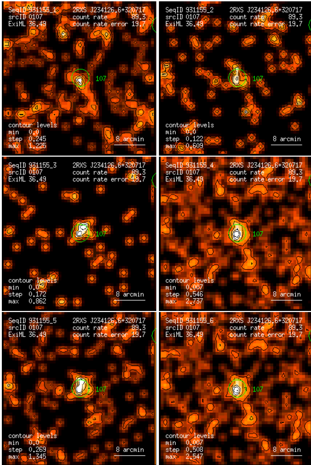
Figure 107: RASS 931155: detection 0107: band rate images, Gaussian filter: (1) PSPC channels 11 – 41, (2) 52 – 90, (3) 91 – 201, (4) 11 – 235, (5) 52 – 201, (6) 11 – 201. Broad band rates in counts/ks. Band rate contour levels in counts/ks/arcmin 2 .
