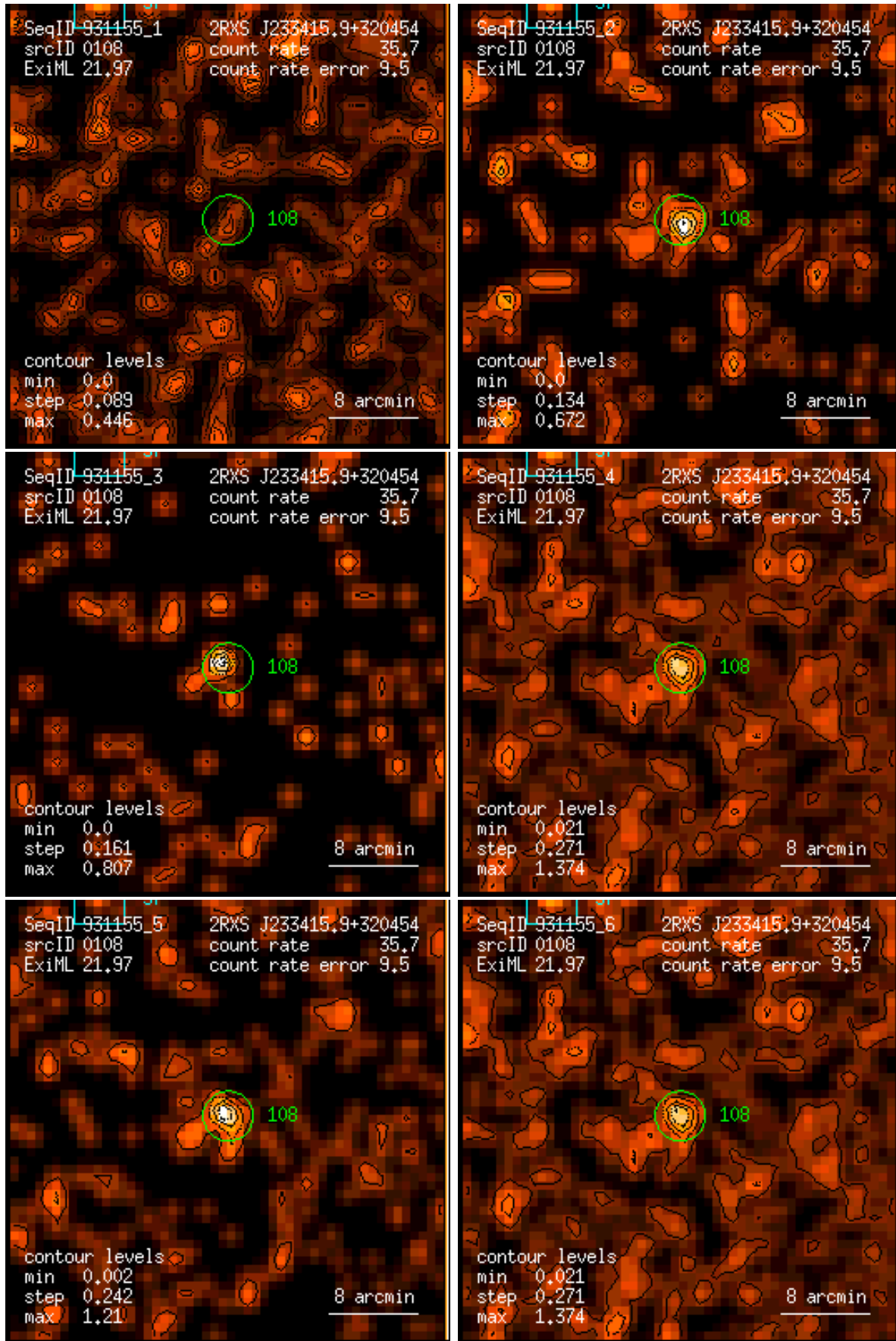
Figure 108: RASS 931155: detection 0108: band rate images, Gaussian filter: (1) PSPC channels 11 – 41, (2) 52 – 90, (3) 91 – 201, (4) 11 – 235, (5) 52 – 201, (6) 11 – 201. Broad band rates in counts/ks. Band rate contour levels in counts/ks/arcmin 2 .
