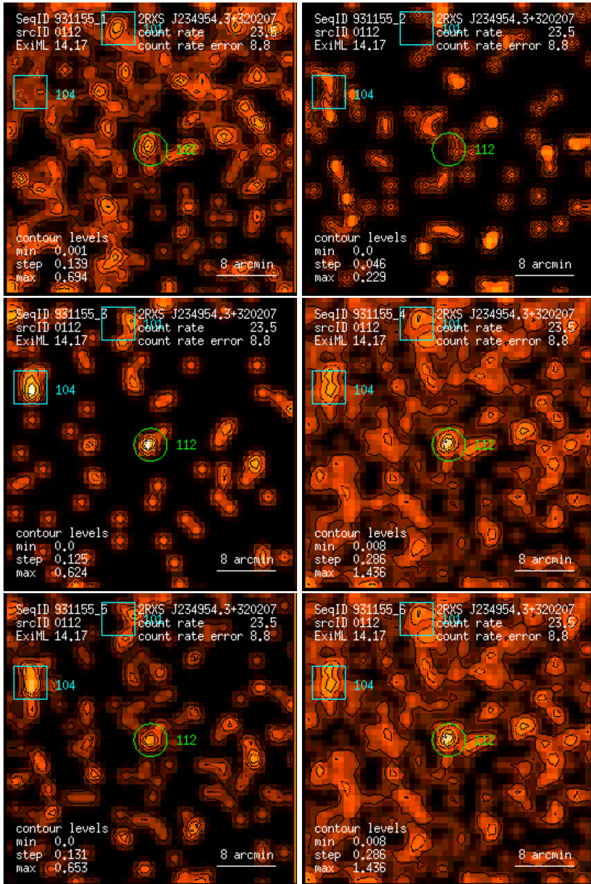
Figure 112: RASS 931155: detection 0112: band rate images, Gaussian filter: (1) PSPC channels 11 – 41, (2) 52 – 90, (3) 91 – 201, (4) 11 – 235, (5) 52 – 201, (6) 11 – 201. Broad band rates in counts/ks. Band rate contour levels in counts/ks/arcmin 2 .
