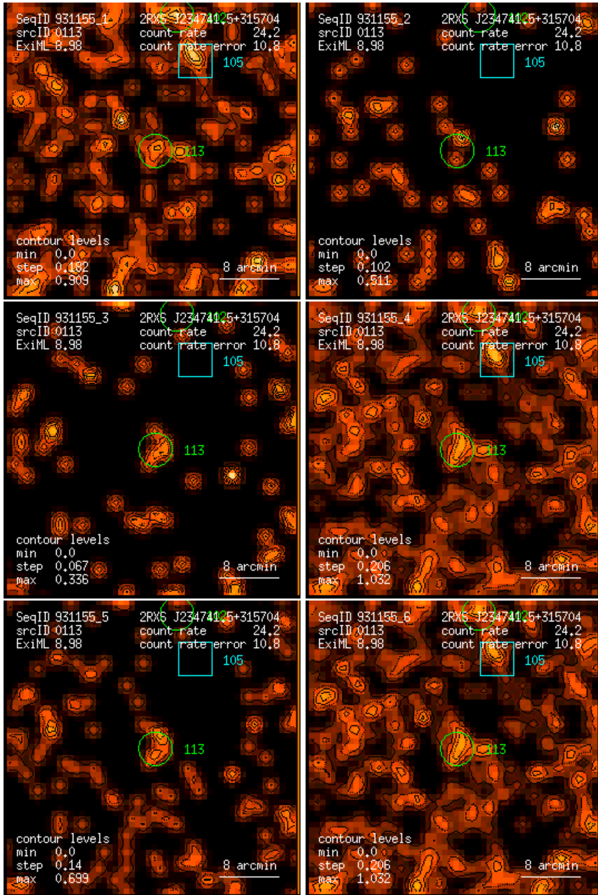
Figure 113: RASS 931155: detection 0113: band rate images, Gaussian filter: (1) PSPC channels 11 – 41, (2) 52 – 90, (3) 91 – 201, (4) 11 – 235, (5) 52 – 201, (6) 11 – 201. Broad band rates in counts/ks. Band rate contour levels in counts/ks/arcmin 2 .
