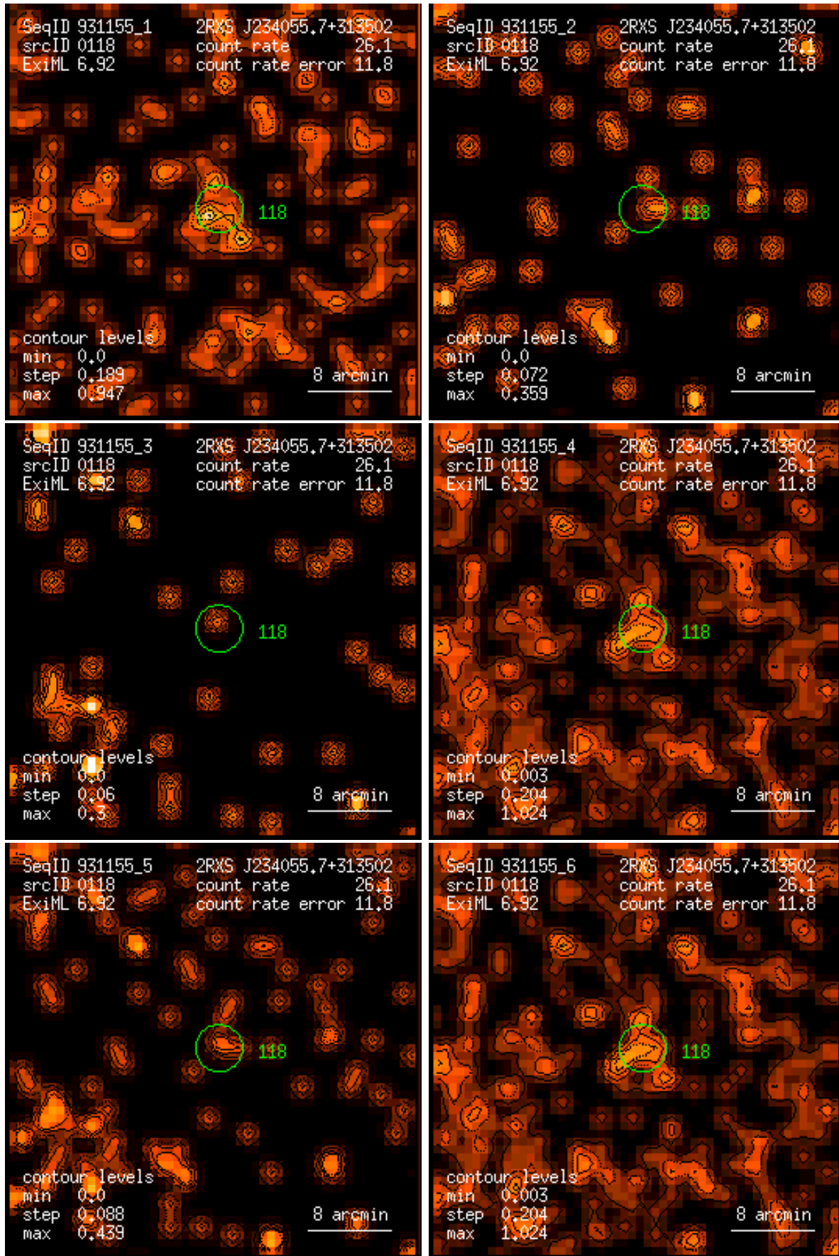
Figure 118: RASS 931155: detection 0118: band rate images, Gaussian filter: (1) PSPC channels 11 – 41, (2) 52 – 90, (3) 91 – 201, (4) 11 – 235, (5) 52 – 201, (6) 11 – 201. Broad band rates in counts/ks. Band rate contour levels in counts/ks/arcmin 2 .
