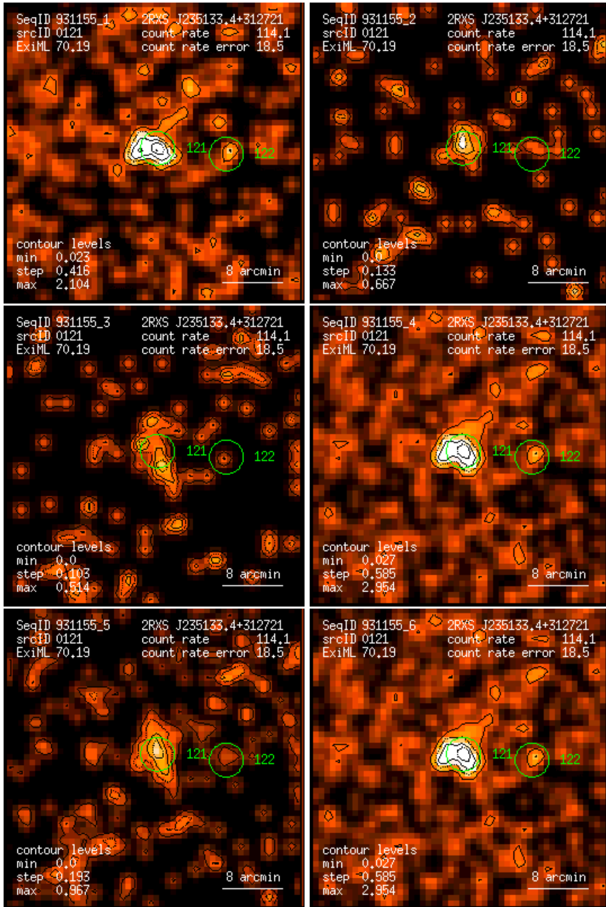
Figure 121: RASS 931155: detection 0121: band rate images, Gaussian filter: (1) PSPC channels 11 – 41, (2) 52 – 90, (3) 91 – 201, (4) 11 – 235, (5) 52 – 201, (6) 11 – 201. Broad band rates in counts/ks. Band rate contour levels in counts/ks/arcmin 2 .
