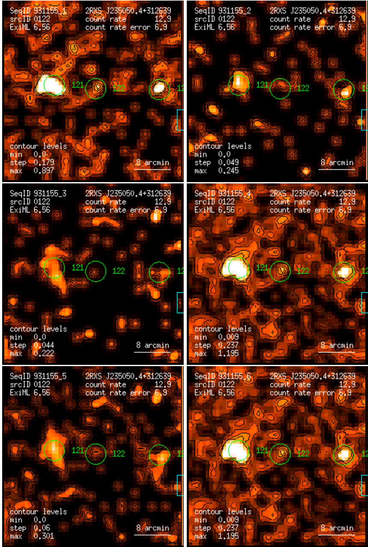
Figure 122: RASS 931155: detection 0122: band rate images, Gaussian filter: (1) PSPC channels 11 – 41, (2) 52 – 90, (3) 91 – 201, (4) 11 – 235, (5) 52 – 201, (6) 11 – 201. Broad band rates in counts/ks. Band rate contour levels in counts/ks/arcmin 2 .
