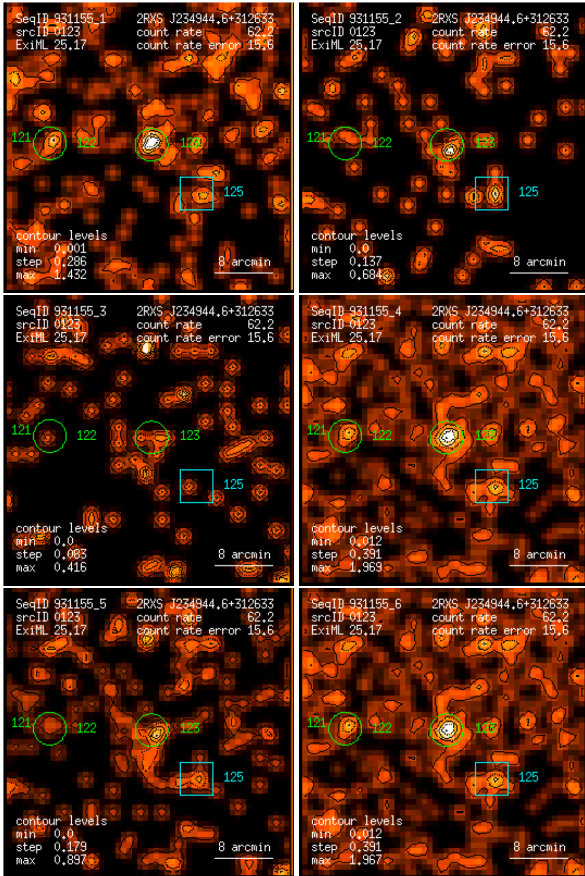
Figure 123: RASS 931155: detection 0123: band rate images, Gaussian filter: (1) PSPC channels 11 – 41, (2) 52 – 90, (3) 91 – 201, (4) 11 – 235, (5) 52 – 201, (6) 11 – 201. Broad band rates in counts/ks. Band rate contour levels in counts/ks/arcmin 2 .
