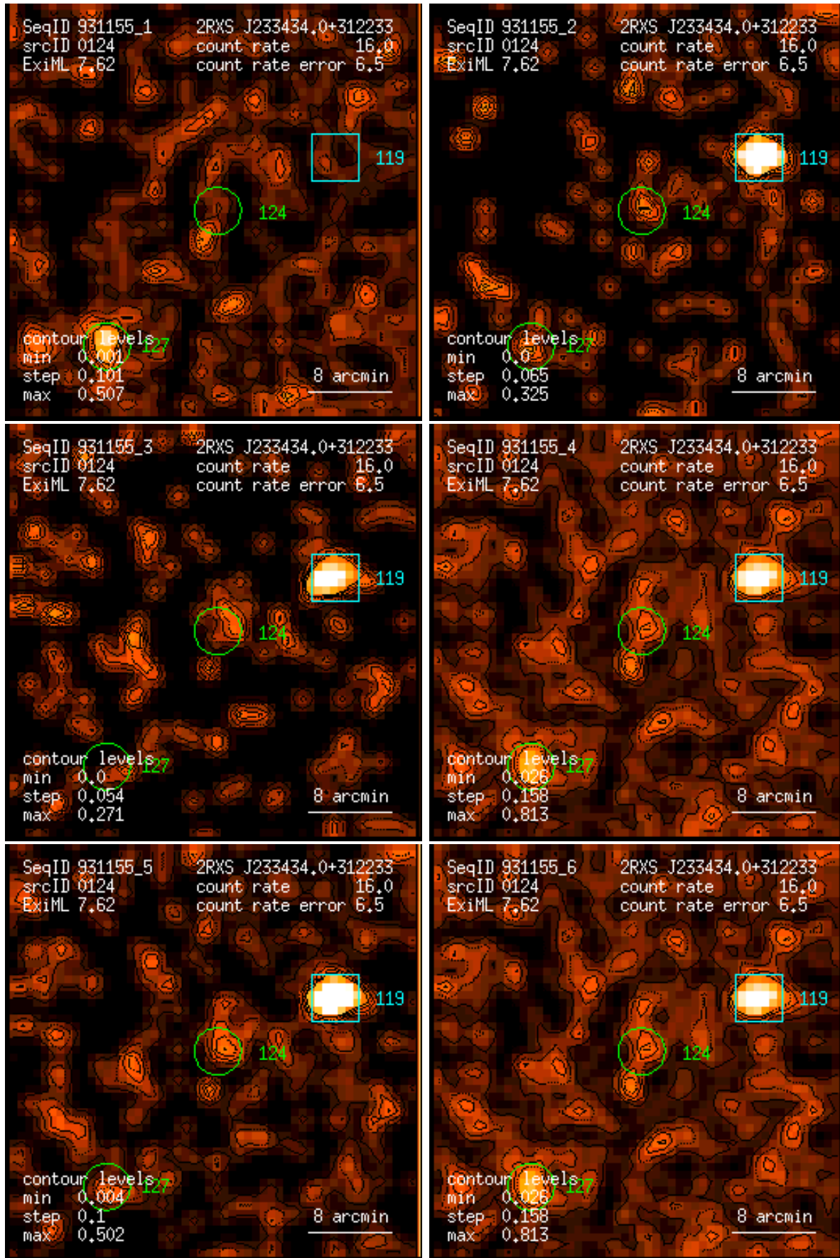
Figure 124: RASS 931155: detection 0124: band rate images, Gaussian filter: (1) PSPC channels 11 – 41, (2) 52 – 90, (3) 91 – 201, (4) 11 – 235, (5) 52 – 201, (6) 11 – 201. Broad band rates in counts/ks. Band rate contour levels in counts/ks/arcmin 2 .
