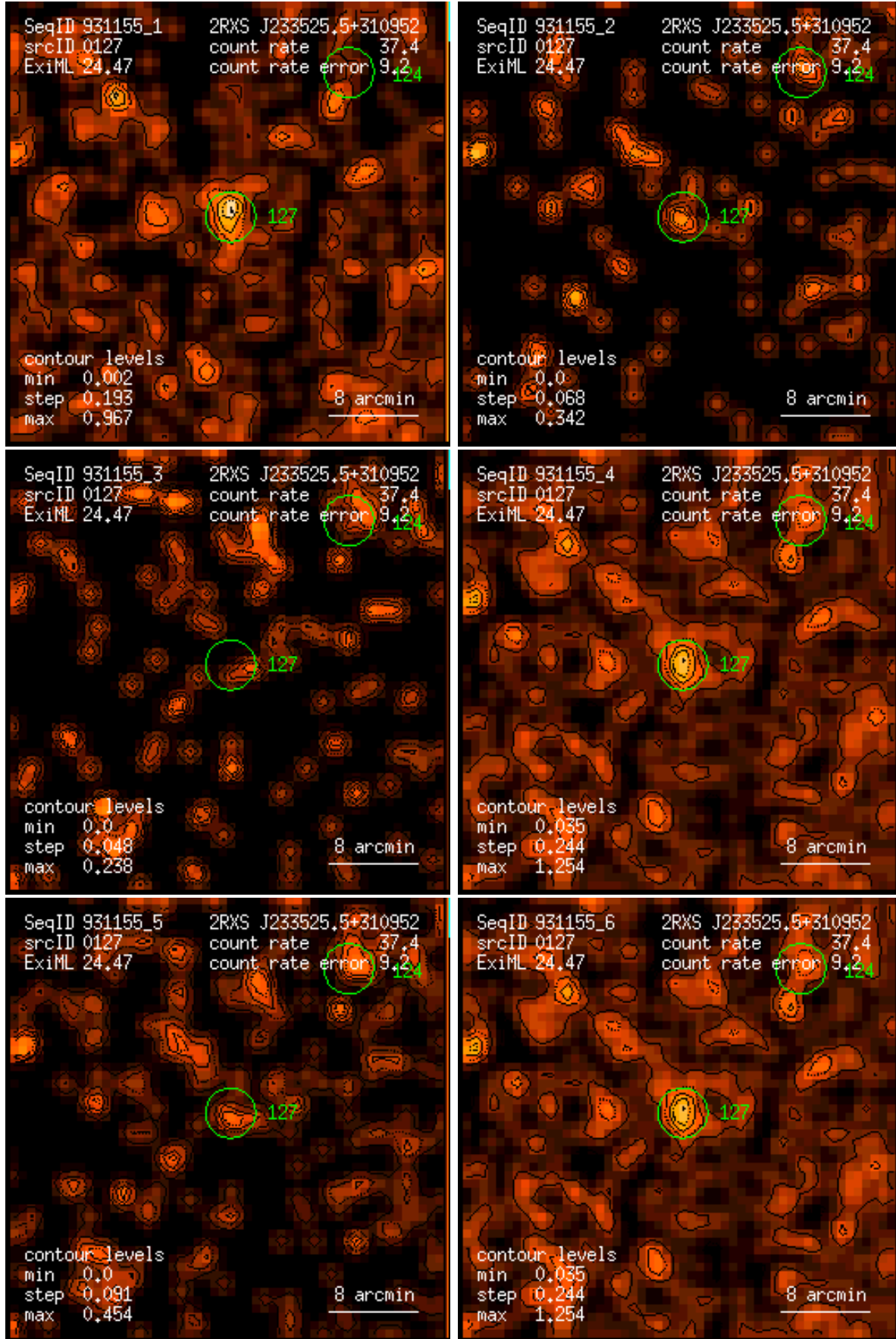
Figure 127: RASS 931155: detection 0127: band rate images, Gaussian filter: (1) PSPC channels 11 – 41, (2) 52 – 90, (3) 91 – 201, (4) 11 – 235, (5) 52 – 201, (6) 11 – 201. Broad band rates in counts/ks. Band rate contour levels in counts/ks/arcmin 2 .
