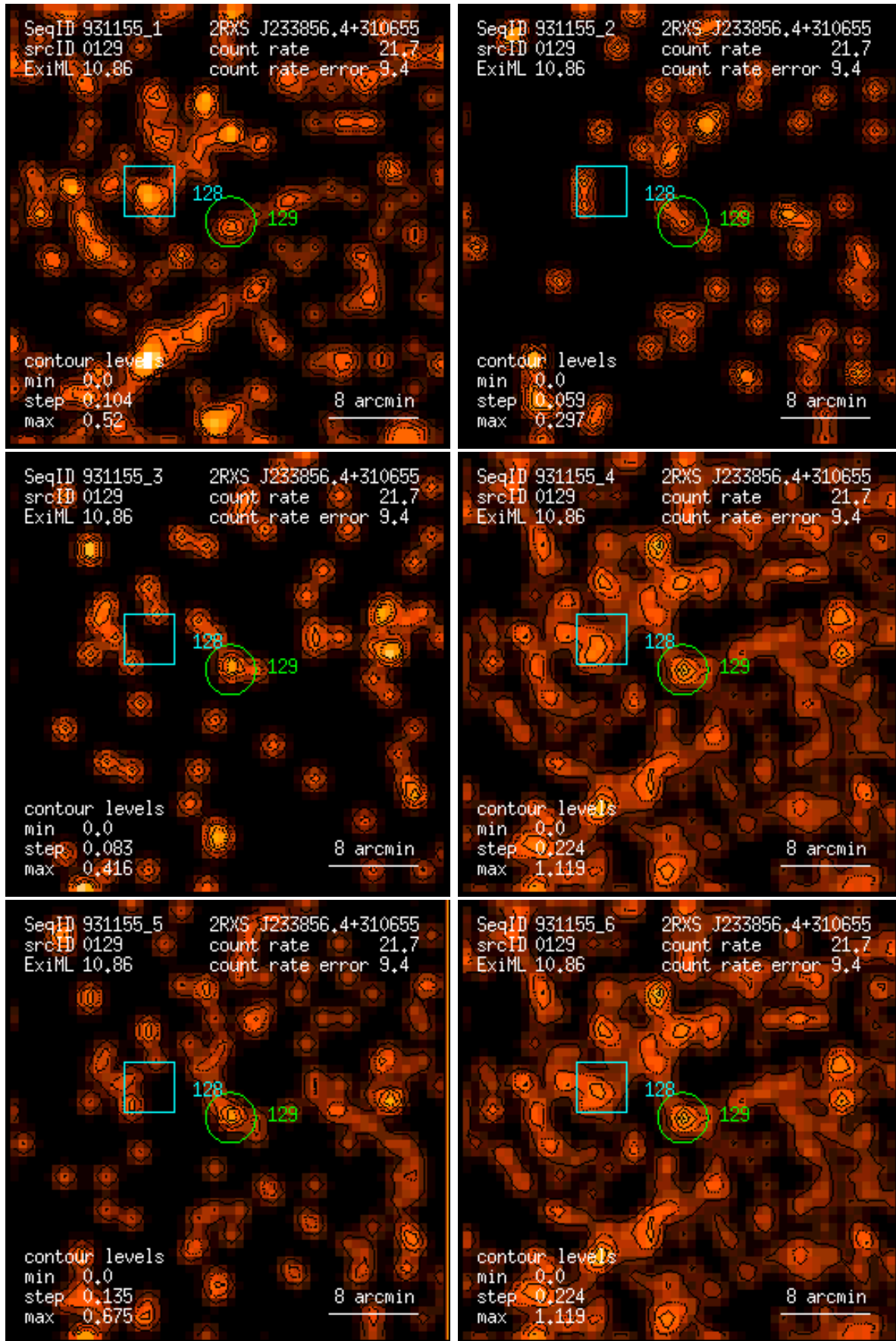
Figure 129: RASS 931155: detection 0129: band rate images, Gaussian filter: (1) PSPC channels 11 – 41, (2) 52 – 90, (3) 91 – 201, (4) 11 – 235, (5) 52 – 201, (6) 11 – 201. Broad band rates in counts/ks. Band rate contour levels in counts/ks/arcmin 2 .
