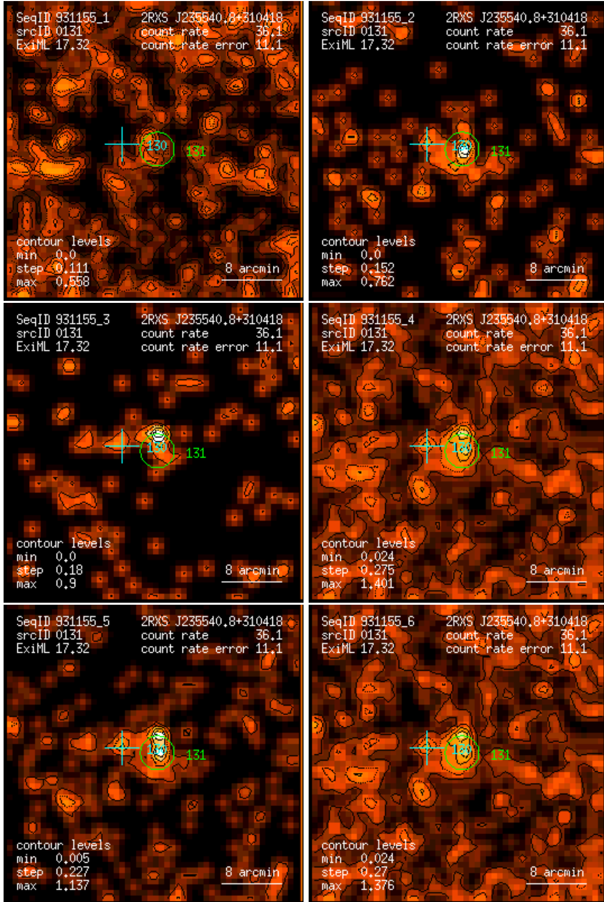
Figure 131: RASS 931155: detection 0131: band rate images, Gaussian filter: (1) PSPC channels 11 – 41, (2) 52 – 90, (3) 91 – 201, (4) 11 – 235, (5) 52 – 201, (6) 11 – 201. Broad band rates in counts/ks. Band rate contour levels in counts/ks/arcmin 2 .
