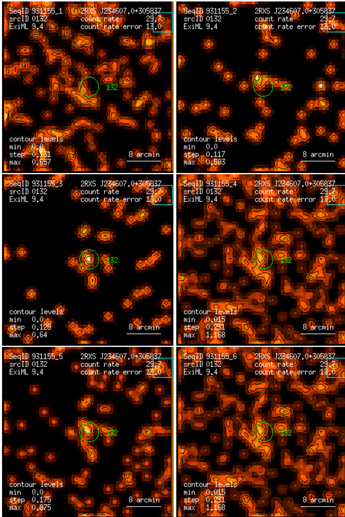
Figure 132: RASS 931155: detection 0132: band rate images, Gaussian filter: (1) PSPC channels 11 – 41, (2) 52 – 90, (3) 91 – 201, (4) 11 – 235, (5) 52 – 201, (6) 11 – 201. Broad band rates in counts/ks. Band rate contour levels in counts/ks/arcmin 2 .
