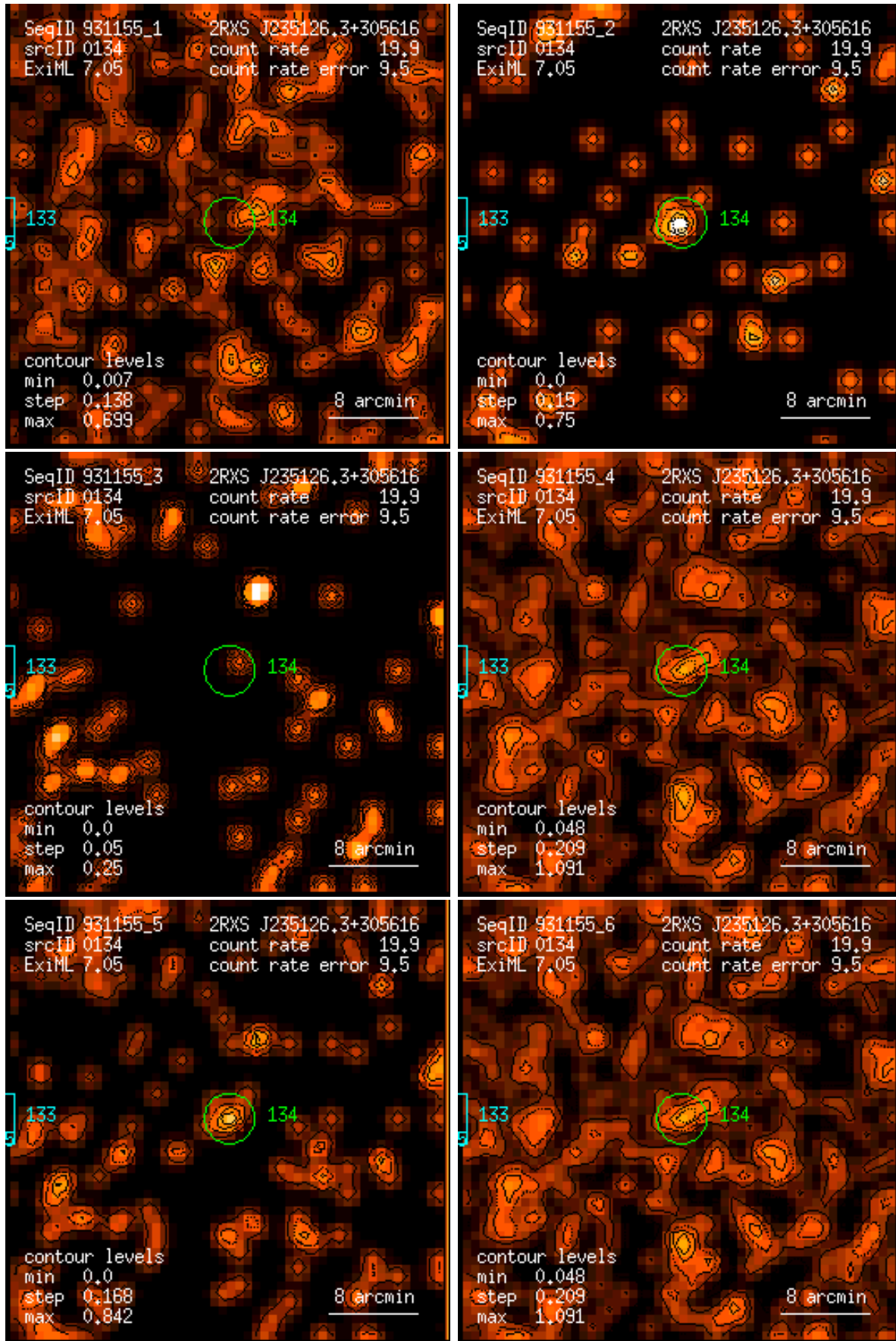
Figure 134: RASS 931155: detection 0134: band rate images, Gaussian filter: (1) PSPC channels 11 – 41, (2) 52 – 90, (3) 91 – 201, (4) 11 – 235, (5) 52 – 201, (6) 11 – 201. Broad band rates in counts/ks. Band rate contour levels in counts/ks/arcmin 2 .
