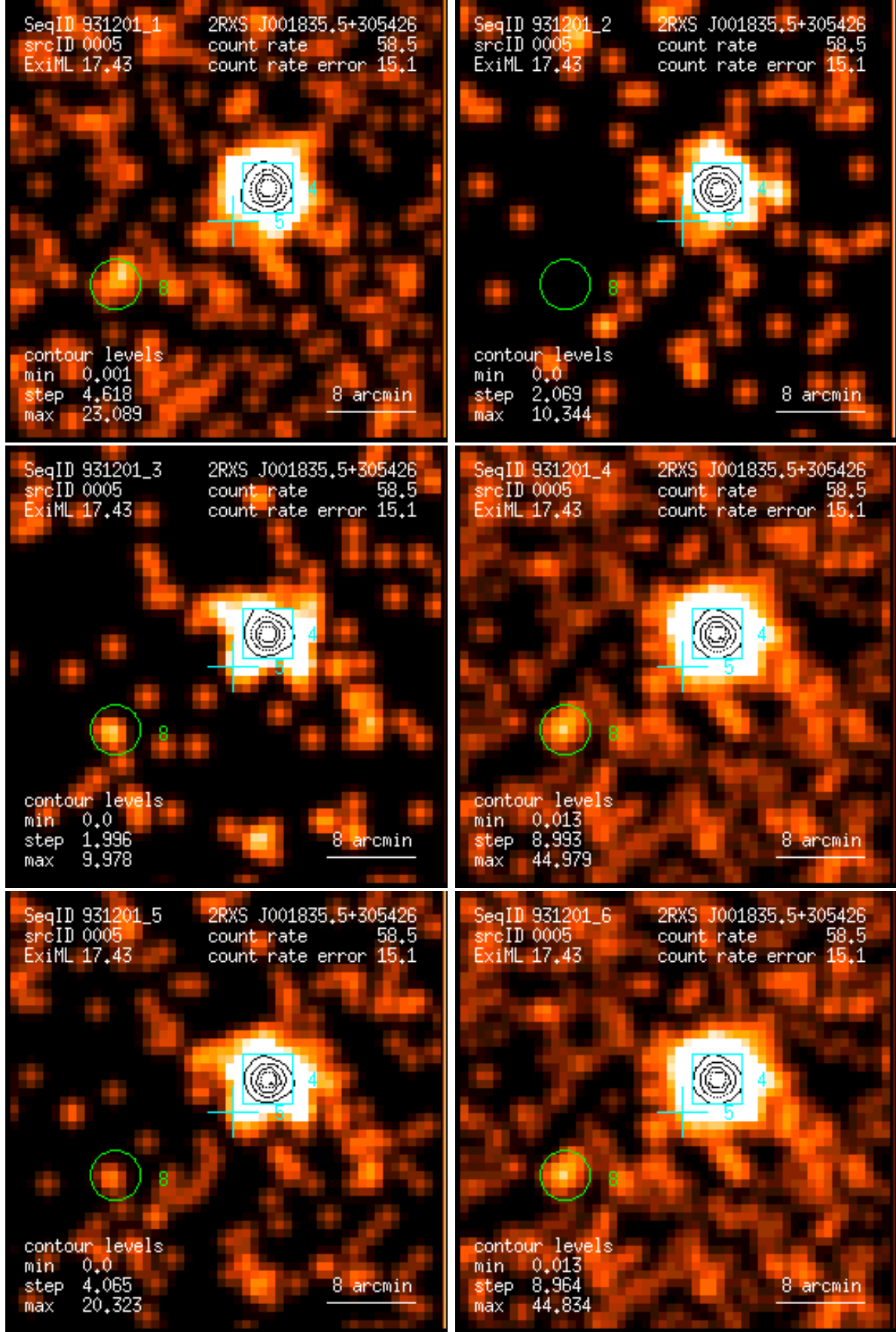
Figure 5: RASS 931201: detection 0005: band rate images, Gaussian filter: (1) PSPC channels 11 – 41, (2) 52 – 90, (3) 91 – 201, (4) 11 – 235, (5) 52 – 201, (6) 11 – 201. Broad band rates in counts/ks. Band rate contour levels in counts/ks/arcmin 2 .
