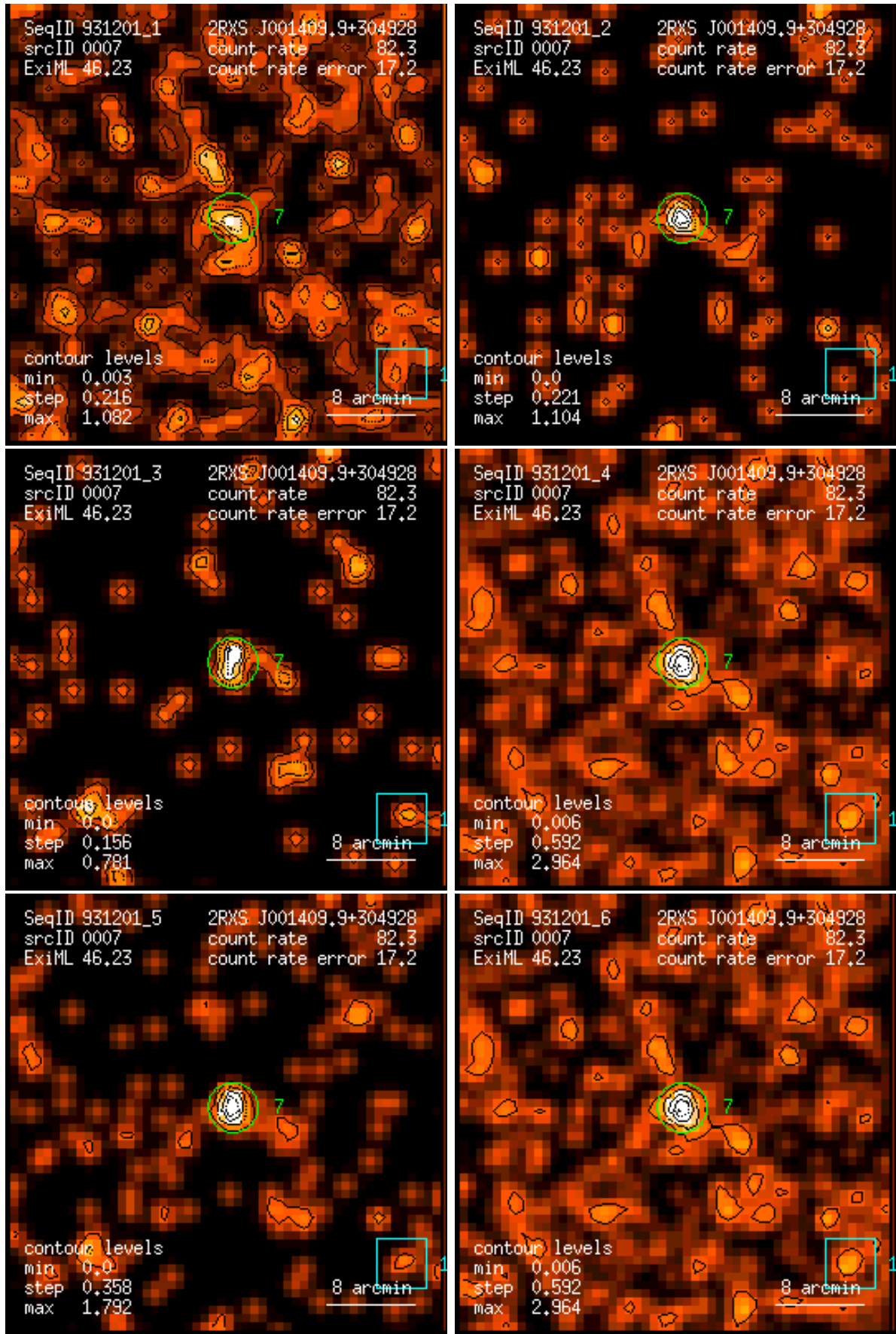
Figure 7: RASS 931201: detection 0007: band rate images, Gaussian filter: (1) PSPC channels 11 – 41, (2) 52 – 90, (3) 91 – 201, (4) 11 – 235, (5) 52 – 201, (6) 11 – 201. Broad band rates in counts/ks. Band rate contour levels in counts/ks/arcmin 2 .
