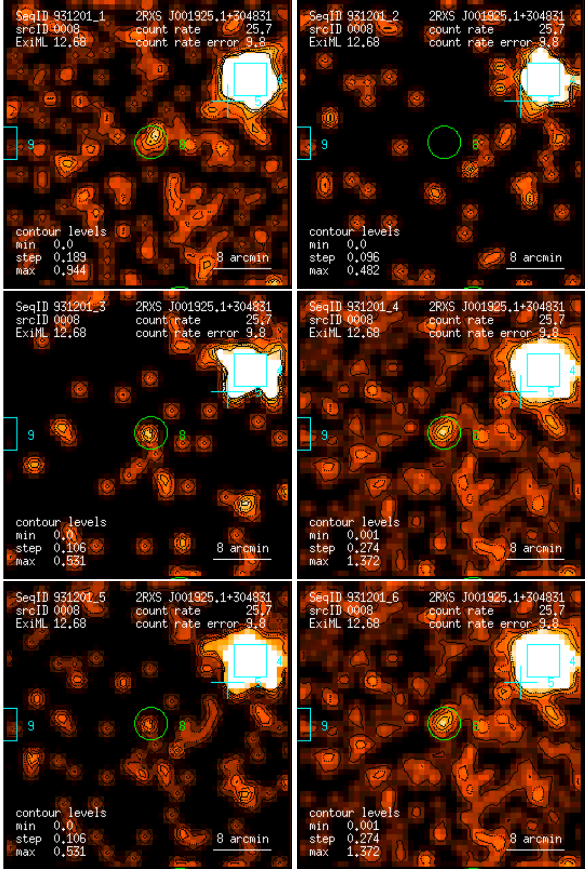
Figure 8: RASS 931201: detection 0008: band rate images, Gaussian filter: (1) PSPC channels 11 – 41, (2) 52 – 90, (3) 91 – 201, (4) 11 – 235, (5) 52 – 201, (6) 11 – 201. Broad band rates in counts/ks. Band rate contour levels in counts/ks/arcmin 2 .
