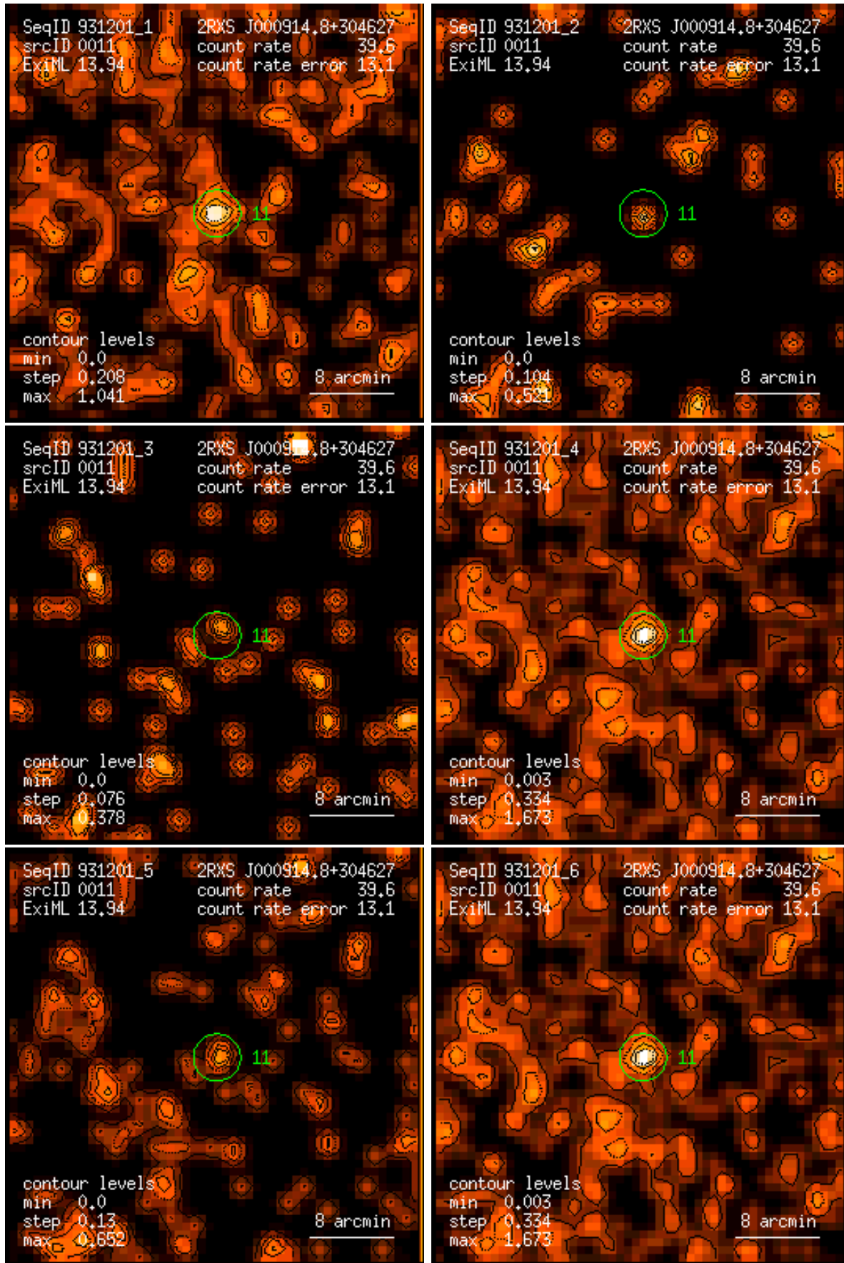
Figure 11: RASS 931201: detection 0011: band rate images, Gaussian filter: (1) PSPC channels 11 – 41, (2) 52 – 90, (3) 91 – 201, (4) 11 – 235, (5) 52 – 201, (6) 11 – 201. Broad band rates in counts/ks. Band rate contour levels in counts/ks/arcmin 2 .
