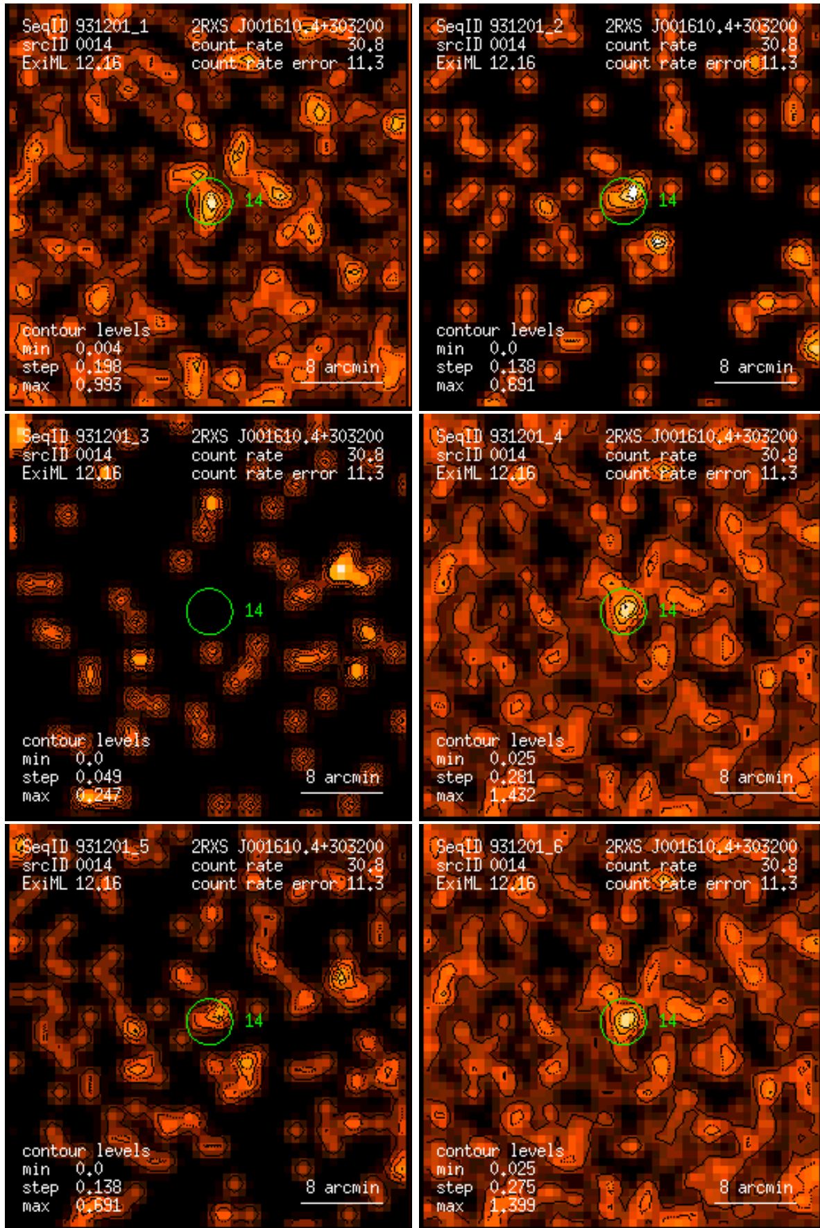
Figure 14: RASS 931201: detection 0014: band rate images, Gaussian filter: (1) PSPC channels 11 – 41, (2) 52 – 90, (3) 91 – 201, (4) 11 – 235, (5) 52 – 201, (6) 11 – 201. Broad band rates in counts/ks. Band rate contour levels in counts/ks/arcmin 2 .
