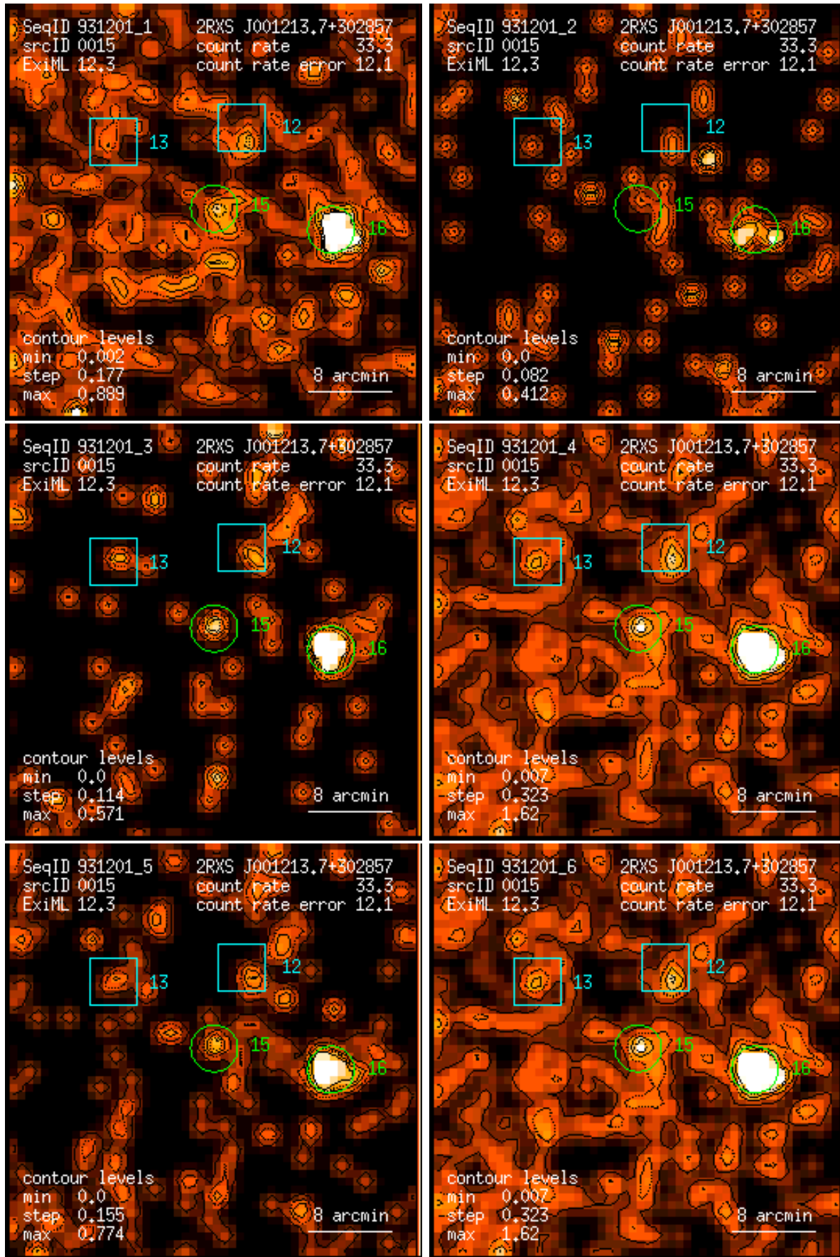
Figure 15: RASS 931201: detection 0015: band rate images, Gaussian filter: (1) PSPC channels 11 – 41, (2) 52 – 90, (3) 91 – 201, (4) 11 – 235, (5) 52 – 201, (6) 11 – 201. Broad band rates in counts/ks. Band rate contour levels in counts/ks/arcmin 2 .
