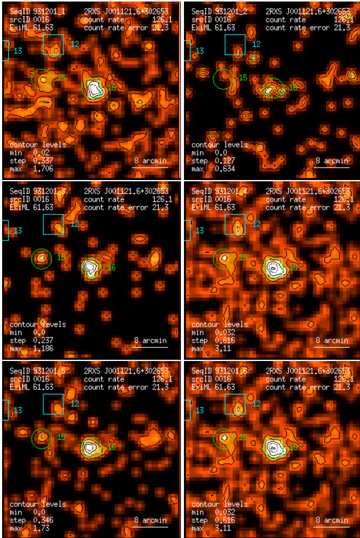
Figure 16: RASS 931201: detection 0016: band rate images, Gaussian filter: (1) PSPC channels 11 – 41, (2) 52 – 90, (3) 91 – 201, (4) 11 – 235, (5) 52 – 201, (6) 11 – 201. Broad band rates in counts/ks. Band rate contour levels in counts/ks/arcmin 2 .
