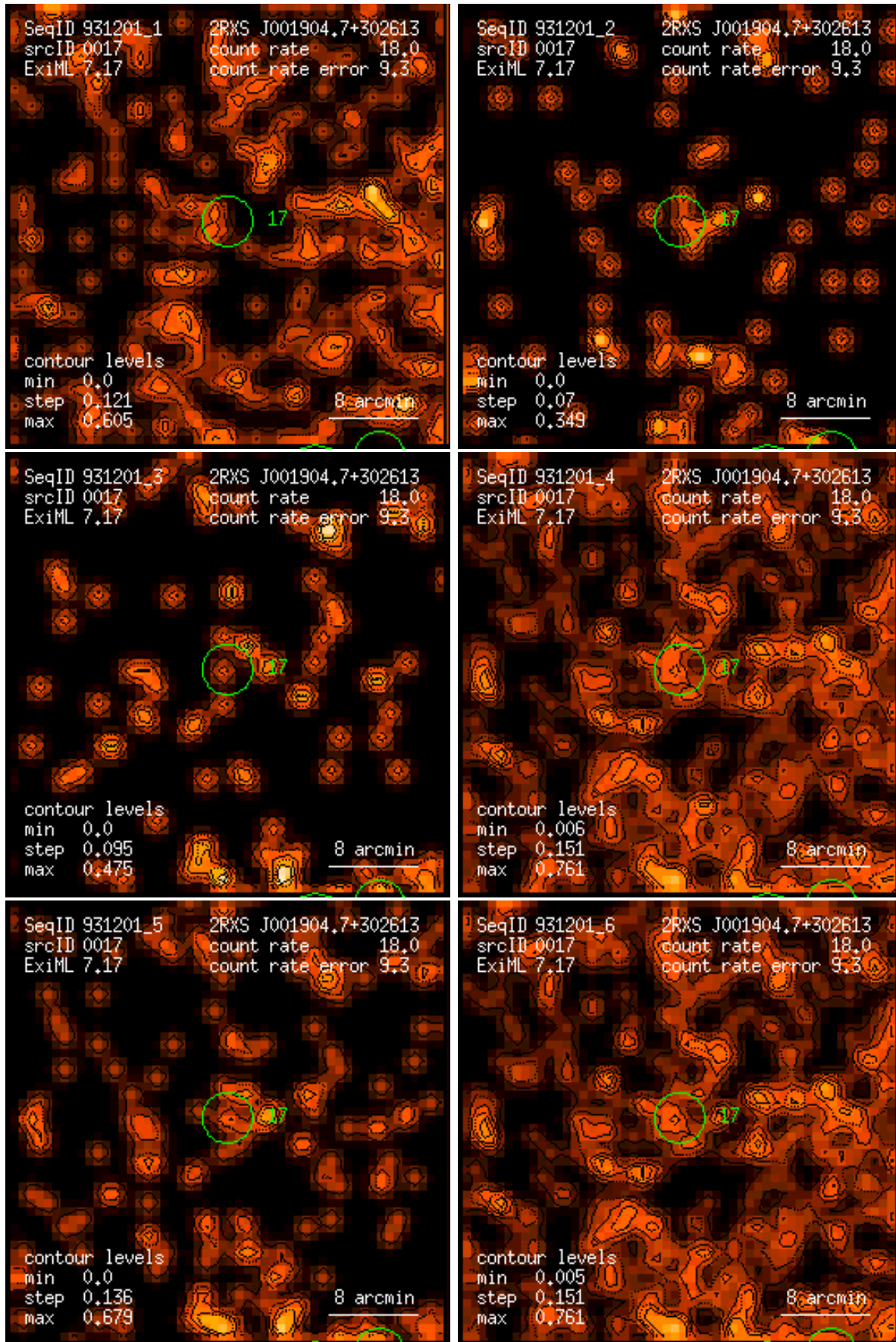
Figure 17: RASS 931201: detection 0017: band rate images, Gaussian filter: (1) PSPC channels 11 – 41, (2) 52 – 90, (3) 91 – 201, (4) 11 – 235, (5) 52 – 201, (6) 11 – 201. Broad band rates in counts/ks. Band rate contour levels in counts/ks/arcmin 2 .
