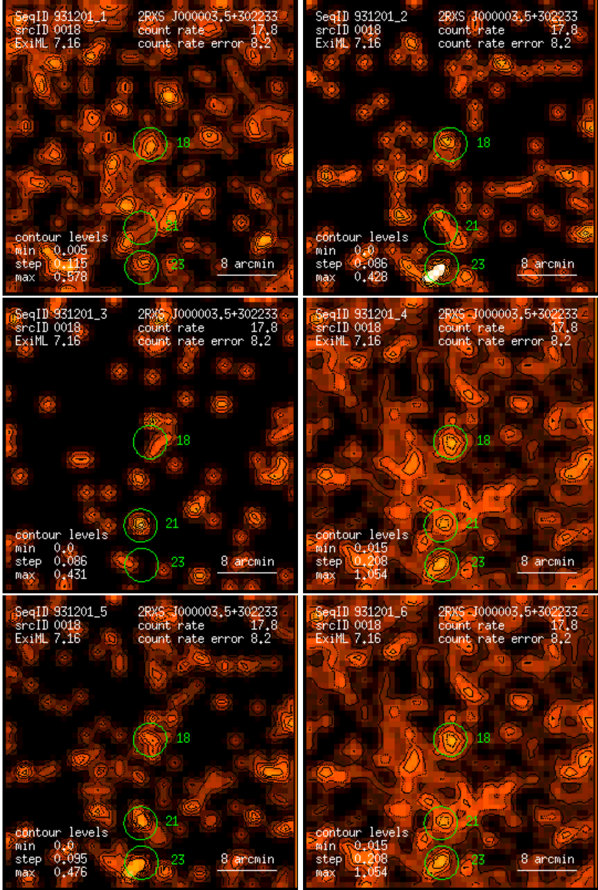
Figure 18: RASS 931201: detection 0018: band rate images, Gaussian filter: (1) PSPC channels 11 – 41, (2) 52 – 90, (3) 91 – 201, (4) 11 – 235, (5) 52 – 201, (6) 11 – 201. Broad band rates in counts/ks. Band rate contour levels in counts/ks/arcmin 2 .
