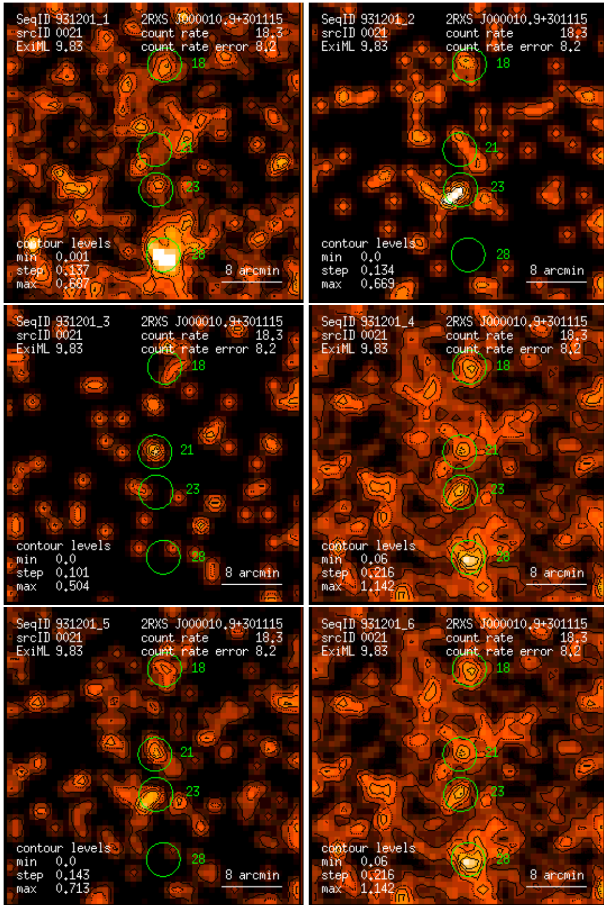
Figure 21: RASS 931201: detection 0021: band rate images, Gaussian filter: (1) PSPC channels 11 – 41, (2) 52 – 90, (3) 91 – 201, (4) 11 – 235, (5) 52 – 201, (6) 11 – 201. Broad band rates in counts/ks. Band rate contour levels in counts/ks/arcmin 2 .
