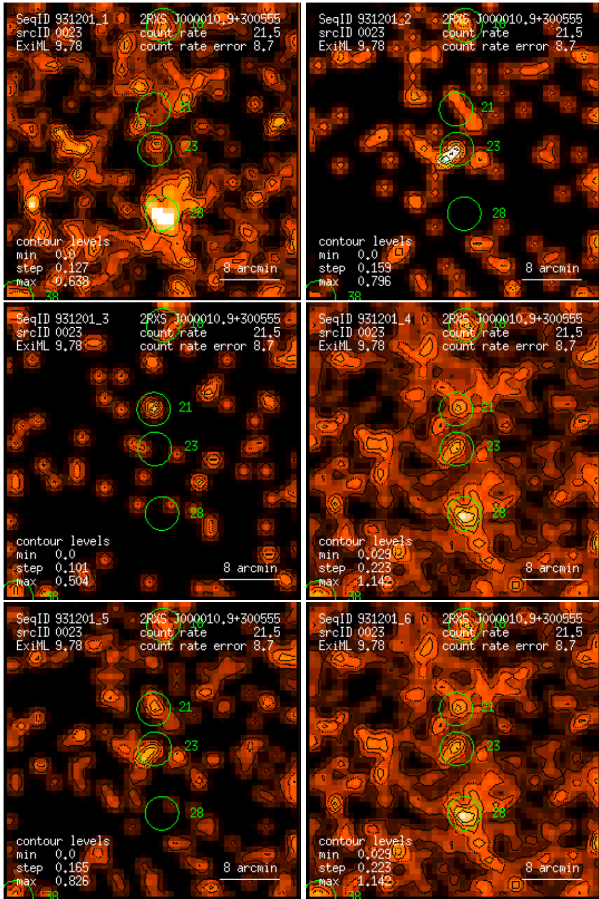
Figure 23: RASS 931201: detection 0023: band rate images, Gaussian filter: (1) PSPC channels 11 – 41, (2) 52 – 90, (3) 91 – 201, (4) 11 – 235, (5) 52 – 201, (6) 11 – 201. Broad band rates in counts/ks. Band rate contour levels in counts/ks/arcmin 2 .
