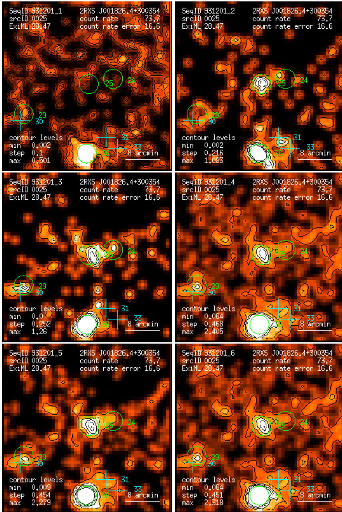
Figure 25: RASS 931201: detection 0025: band rate images, Gaussian filter: (1) PSPC channels 11 – 41, (2) 52 – 90, (3) 91 – 201, (4) 11 – 235, (5) 52 – 201, (6) 11 – 201. Broad band rates in counts/ks. Band rate contour levels in counts/ks/arcmin 2 .
