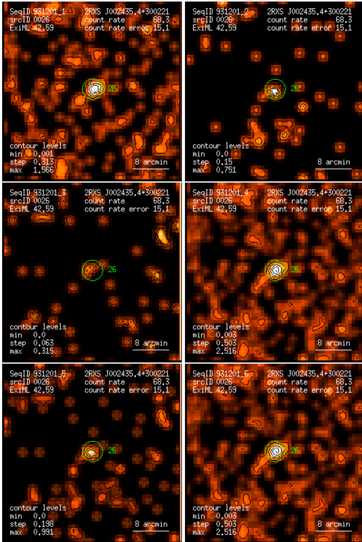
Figure 26: RASS 931201: detection 0026: band rate images, Gaussian filter: (1) PSPC channels 11 – 41, (2) 52 – 90, (3) 91 – 201, (4) 11 – 235, (5) 52 – 201, (6) 11 – 201. Broad band rates in counts/ks. Band rate contour levels in counts/ks/arcmin 2 .
