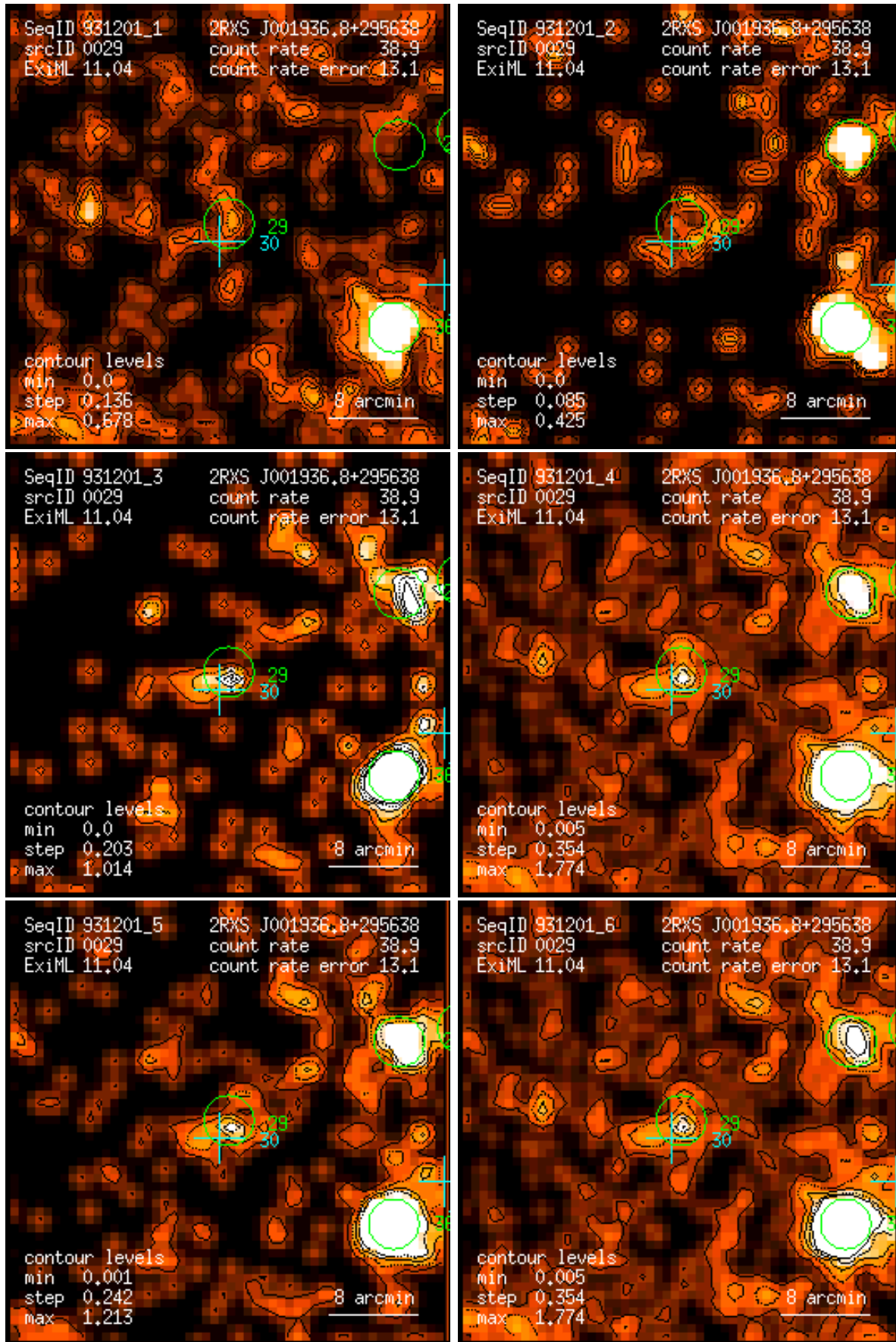
Figure 29: RASS 931201: detection 0029: band rate images, Gaussian filter: (1) PSPC channels 11 – 41, (2) 52 – 90, (3) 91 – 201, (4) 11 – 235, (5) 52 – 201, (6) 11 – 201. Broad band rates in counts/ks. Band rate contour levels in counts/ks/arcmin 2 .
