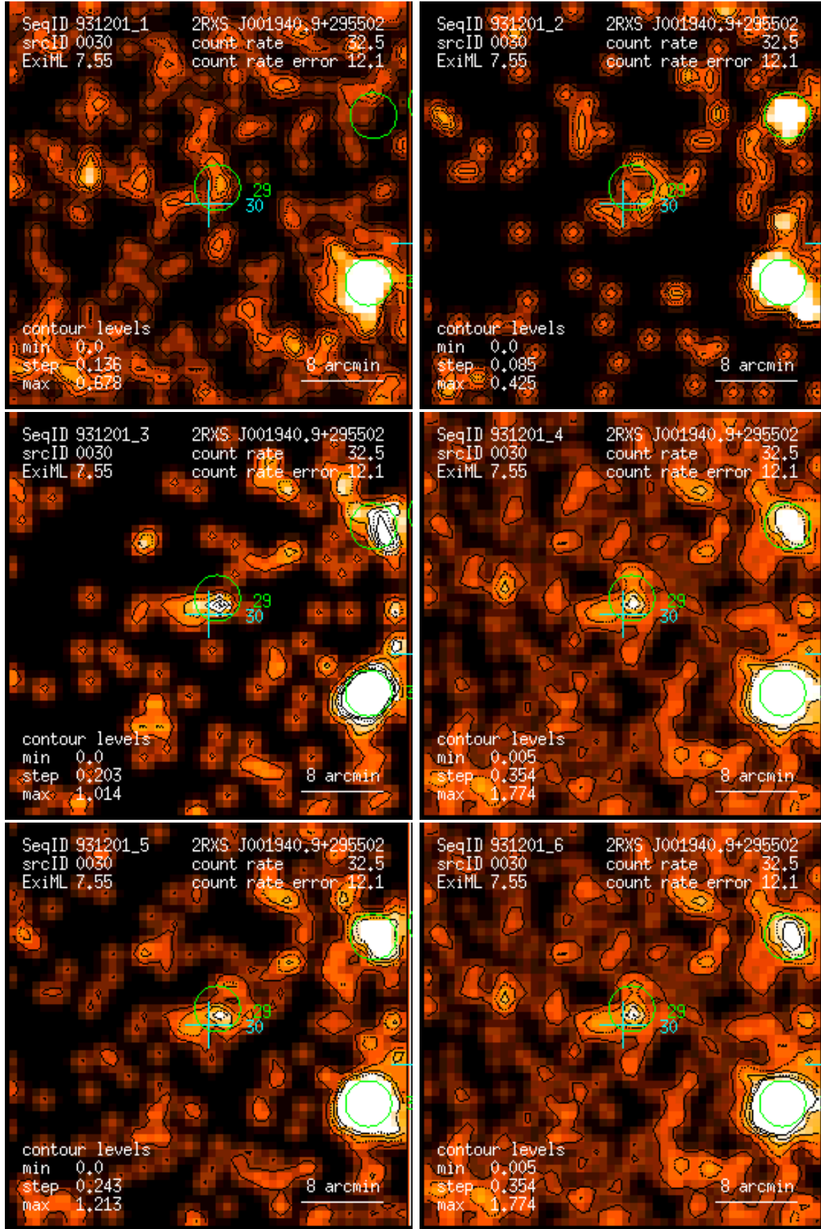
Figure 30: RASS 931201: detection 0030: band rate images, Gaussian filter: (1) PSPC channels 11 – 41, (2) 52 – 90, (3) 91 – 201, (4) 11 – 235, (5) 52 – 201, (6) 11 – 201. Broad band rates in counts/ks. Band rate contour levels in counts/ks/arcmin 2 .
