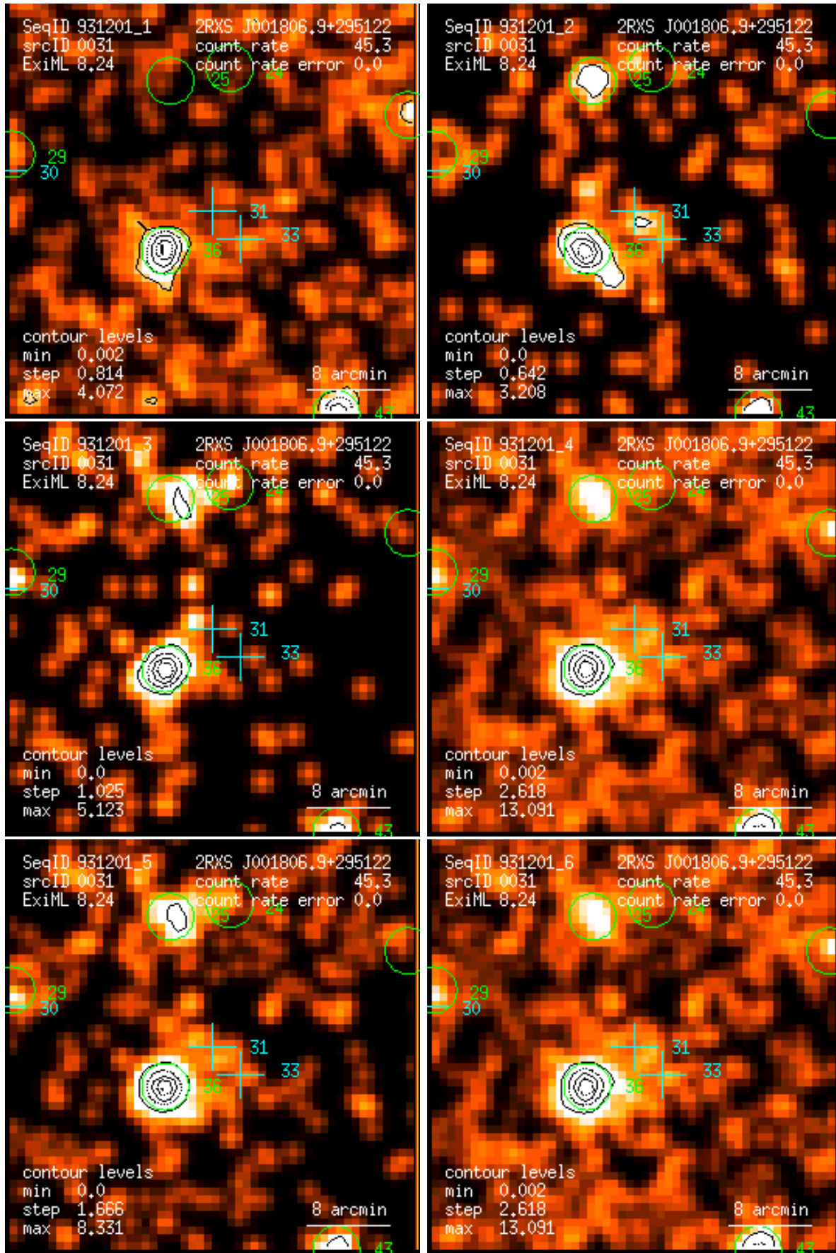
Figure 31: RASS 931201: detection 0031: band rate images, Gaussian filter: (1) PSPC channels 11 – 41, (2) 52 – 90, (3) 91 – 201, (4) 11 – 235, (5) 52 – 201, (6) 11 – 201. Broad band rates in counts/ks. Band rate contour levels in counts/ks/arcmin 2 .
