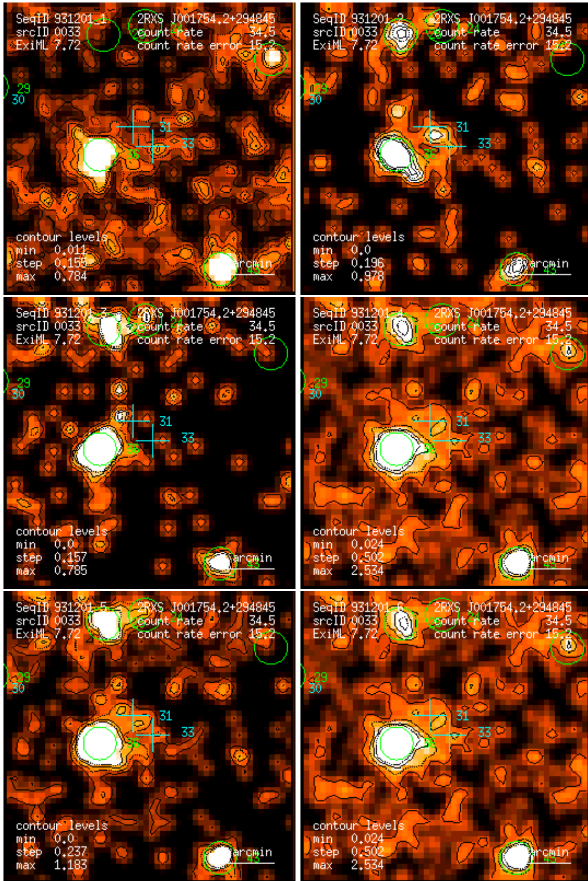
Figure 33: RASS 931201: detection 0033: band rate images, Gaussian filter: (1) PSPC channels 11 – 41, (2) 52 – 90, (3) 91 – 201, (4) 11 – 235, (5) 52 – 201, (6) 11 – 201. Broad band rates in counts/ks. Band rate contour levels in counts/ks/arcmin 2 .
