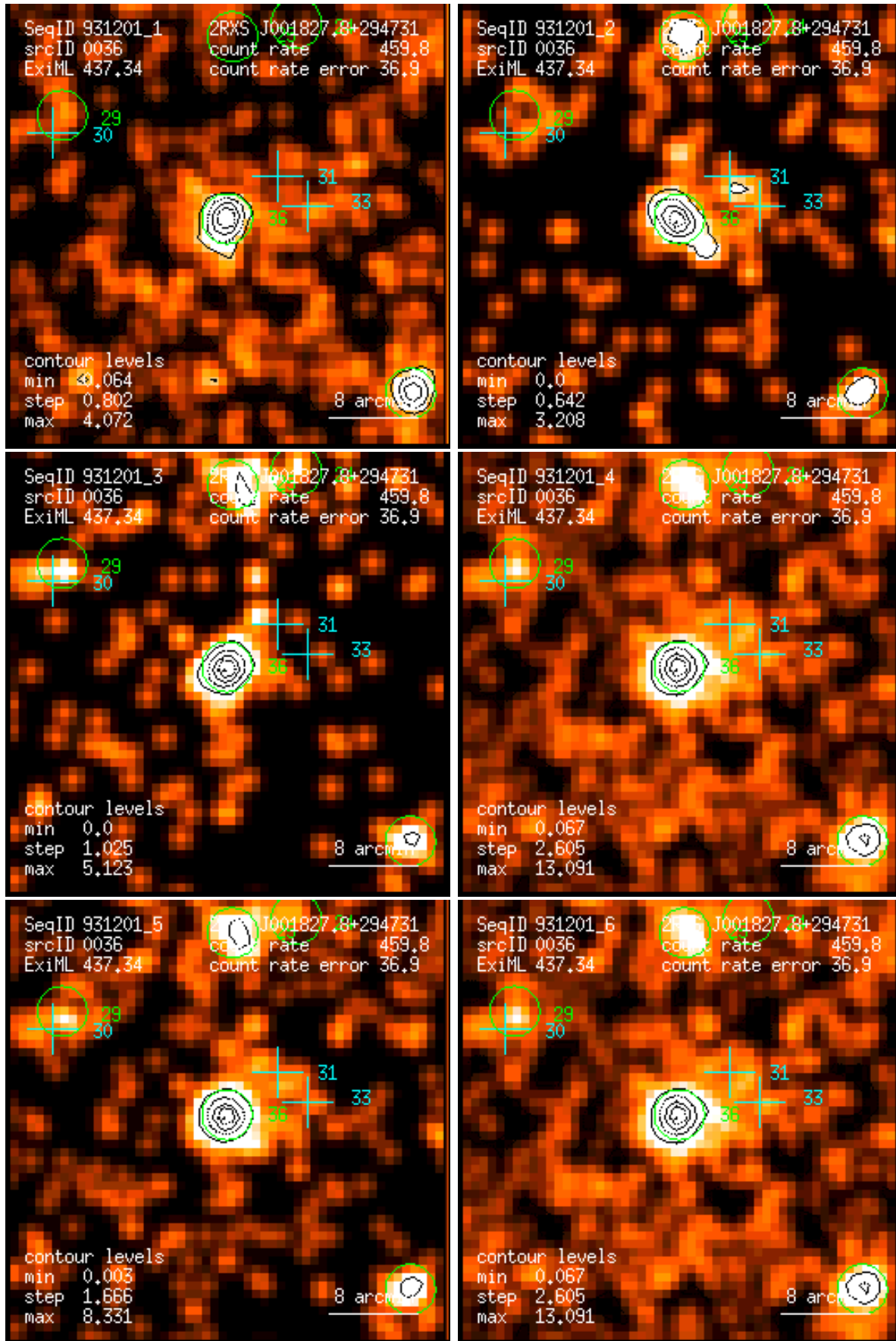
Figure 36: RASS 931201: detection 0036: band rate images, Gaussian filter: (1) PSPC channels 11 – 41, (2) 52 – 90, (3) 91 – 201, (4) 11 – 235, (5) 52 – 201, (6) 11 – 201. Broad band rates in counts/ks. Band rate contour levels in counts/ks/arcmin 2 .
