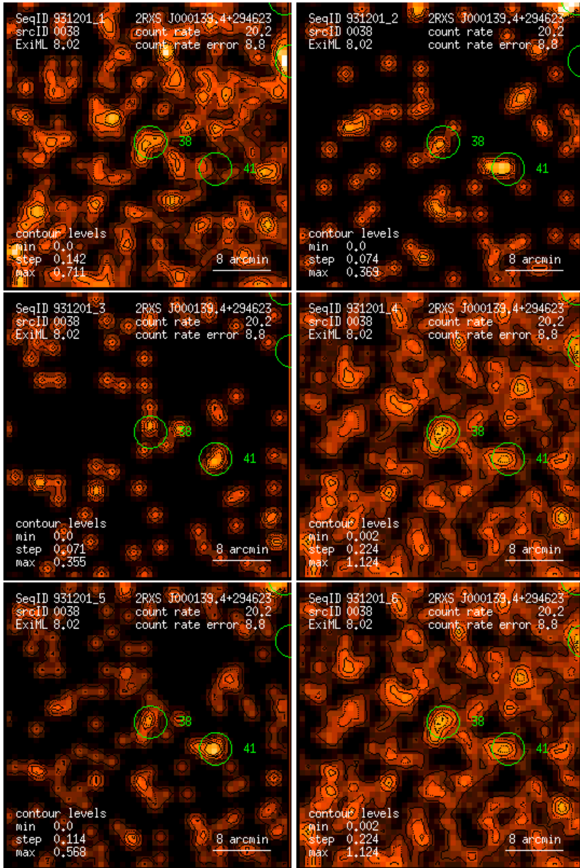
Figure 38: RASS 931201: detection 0038: band rate images, Gaussian filter: (1) PSPC channels 11 – 41, (2) 52 – 90, (3) 91 – 201, (4) 11 – 235, (5) 52 – 201, (6) 11 – 201. Broad band rates in counts/ks. Band rate contour levels in counts/ks/arcmin 2 .
