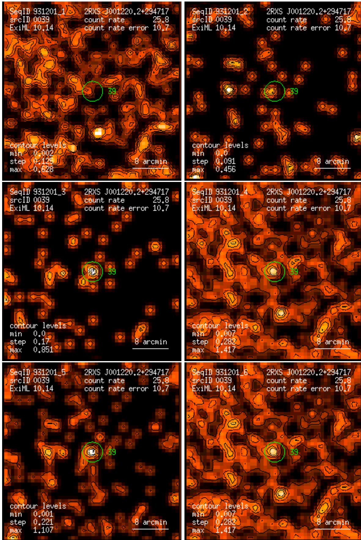
Figure 39: RASS 931201: detection 0039: band rate images, Gaussian filter: (1) PSPC channels 11 – 41, (2) 52 – 90, (3) 91 – 201, (4) 11 – 235, (5) 52 – 201, (6) 11 – 201. Broad band rates in counts/ks. Band rate contour levels in counts/ks/arcmin 2 .
