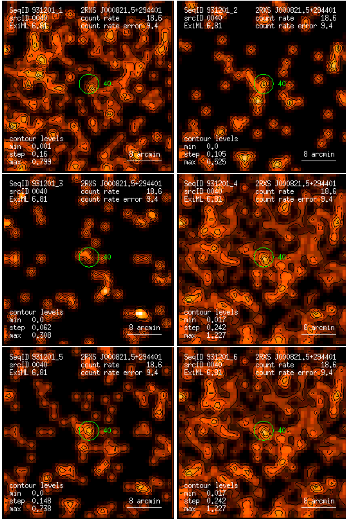
Figure 40: RASS 931201: detection 0040: band rate images, Gaussian filter: (1) PSPC channels 11 – 41, (2) 52 – 90, (3) 91 – 201, (4) 11 – 235, (5) 52 – 201, (6) 11 – 201. Broad band rates in counts/ks. Band rate contour levels in counts/ks/arcmin 2 .
